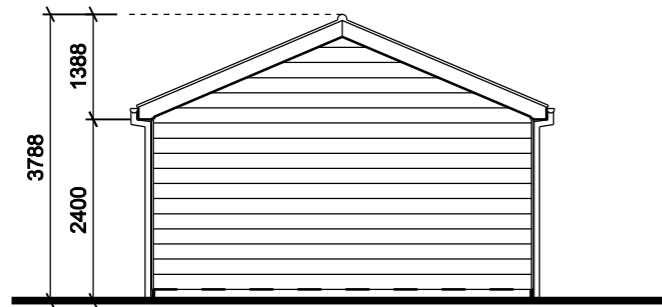
SIDE ELEVATION
