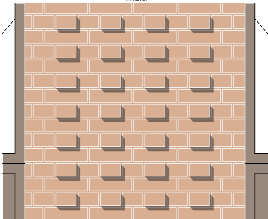
Red Brick Type B: English Bond With Projecting Headers - Wienerberger Washington Red Multi
