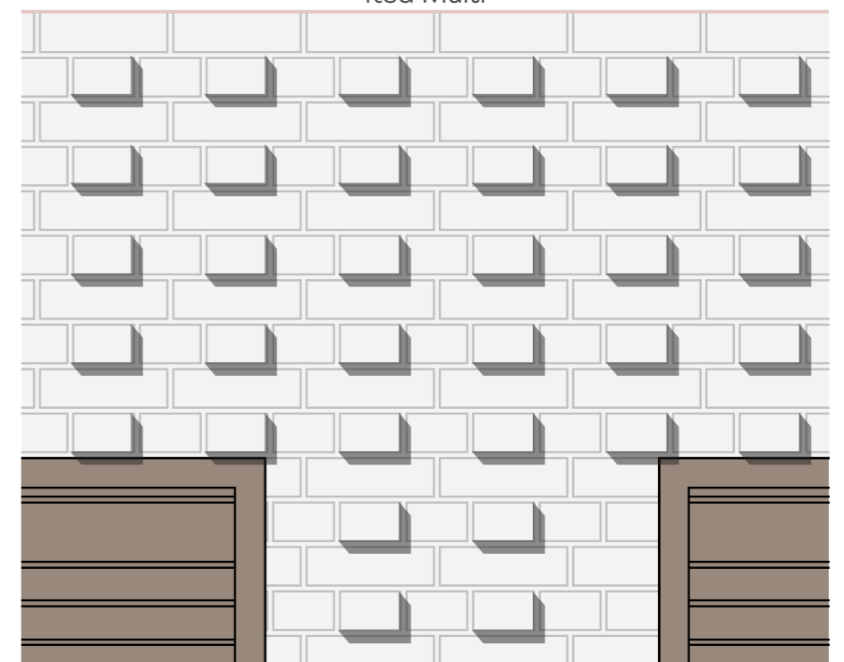
Brick Type D: English Bond With Projecting Headers - Camtech All White Bromo
