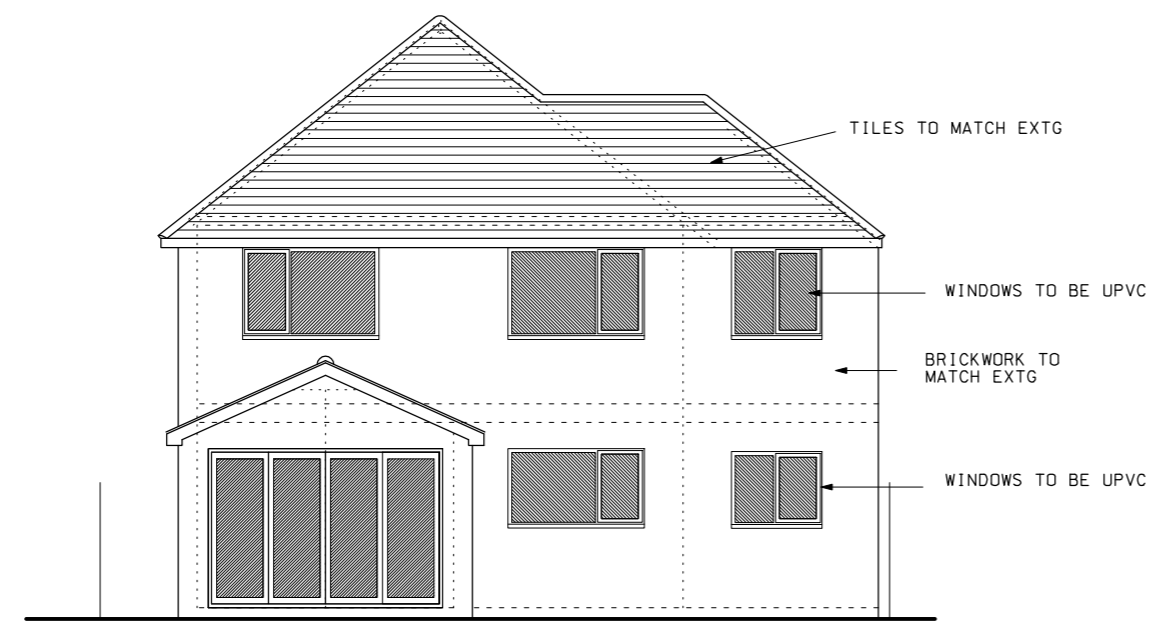
Rear Elevation
