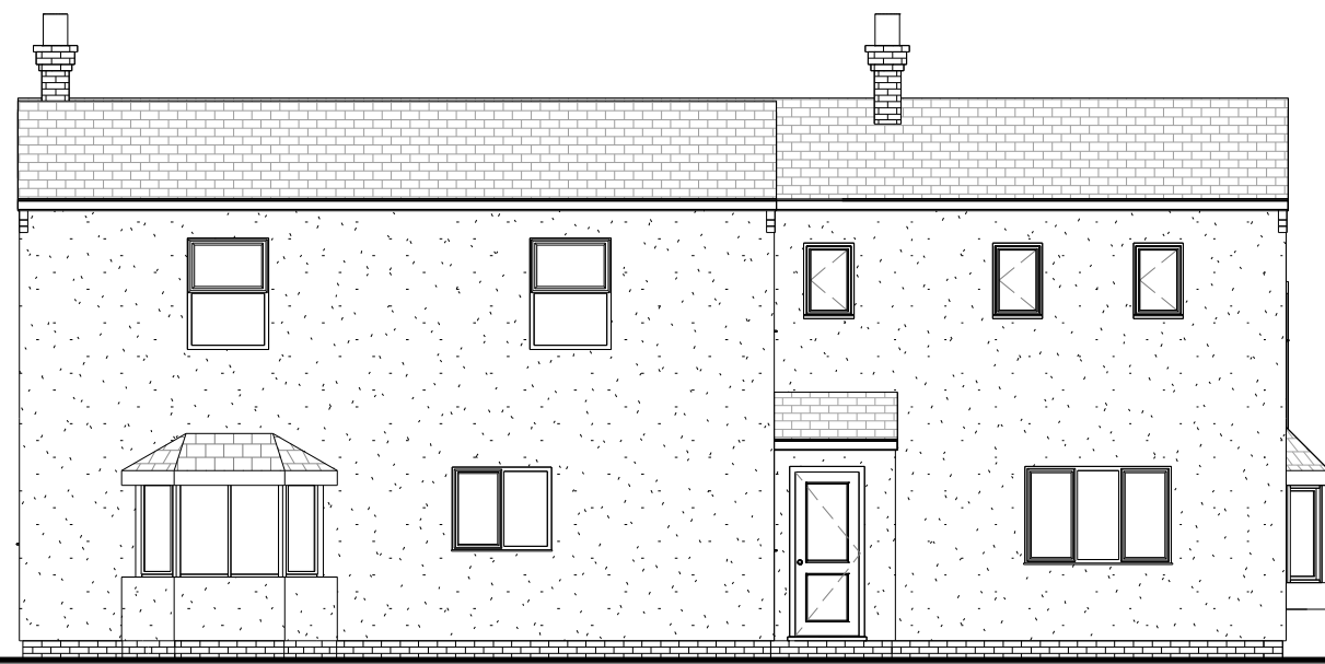
2 Existing - South Elevation 1 : 100
