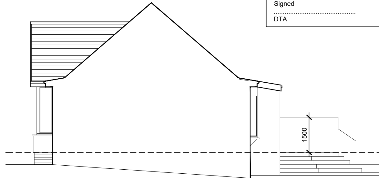
Side Elevation
