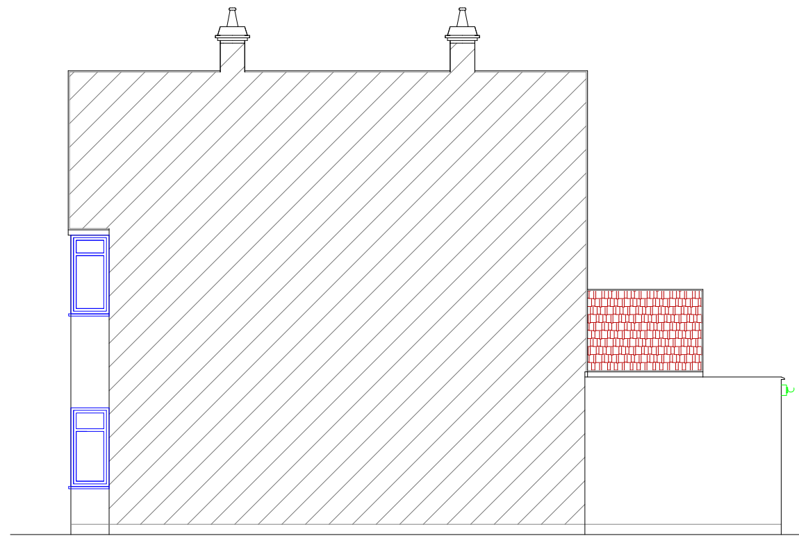
EXISTING RIGHT SIDE VIEW
