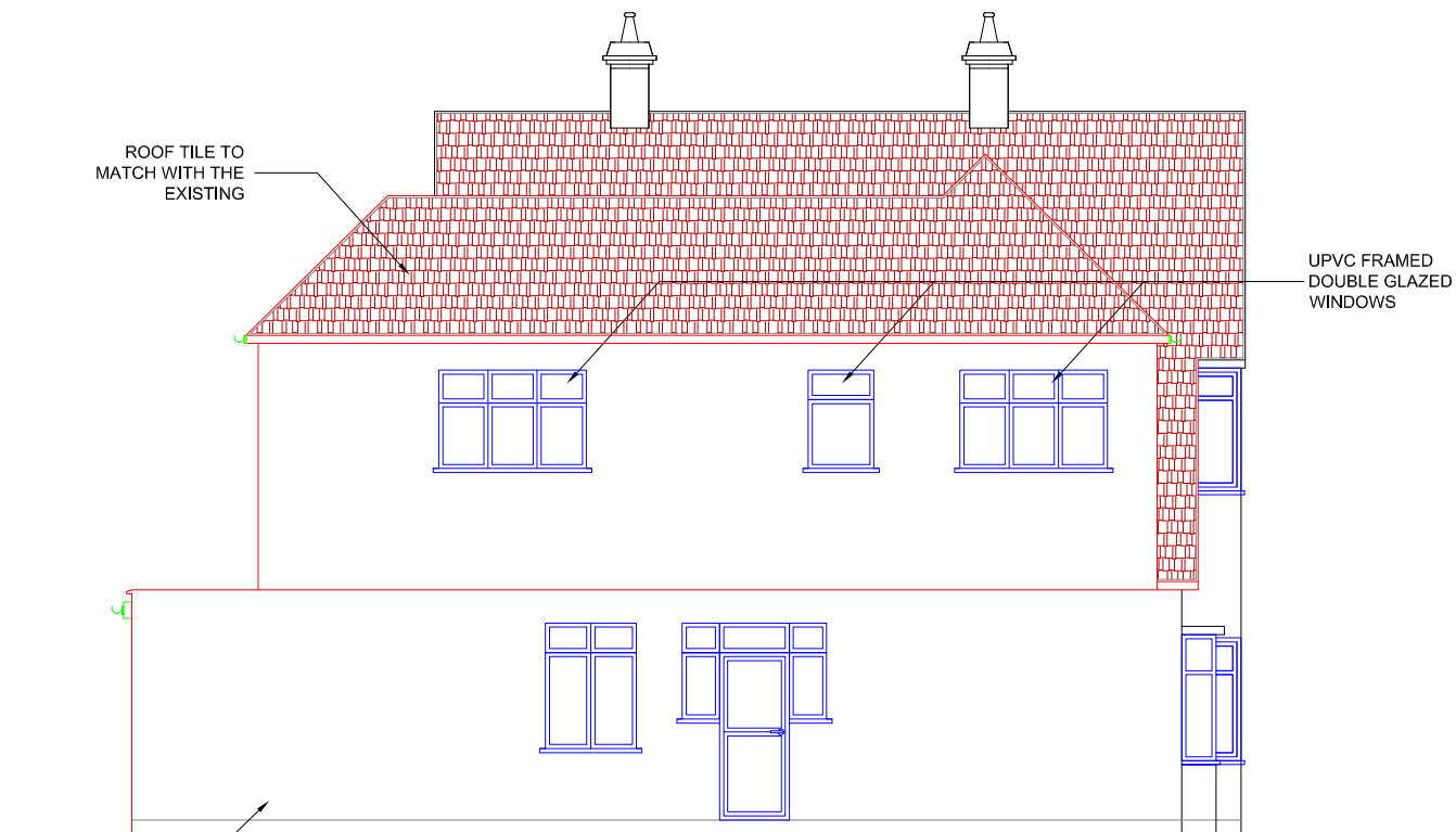
PROPOSED LEFT SIDE VIEW
