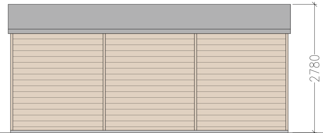
EAST ELEVATION
