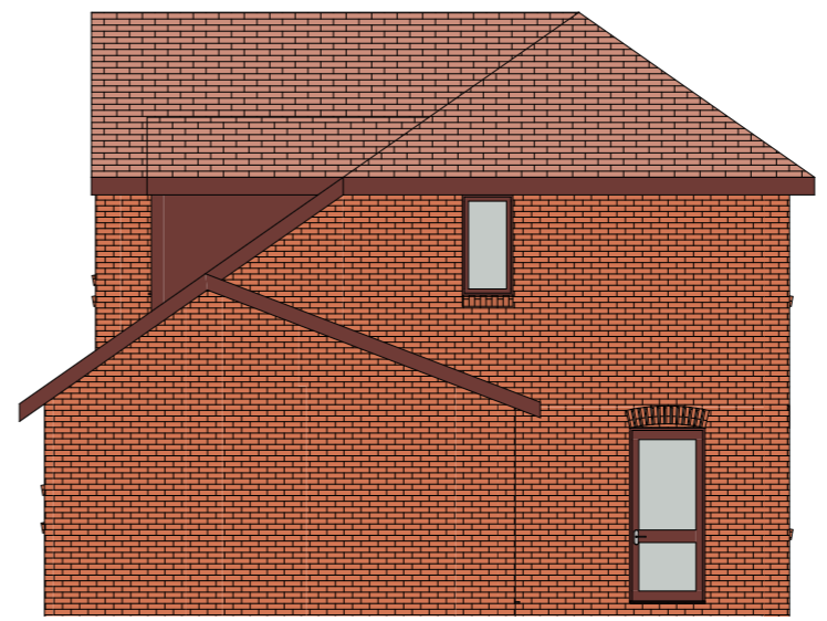
2 Proposed Side Elevation 1:100
