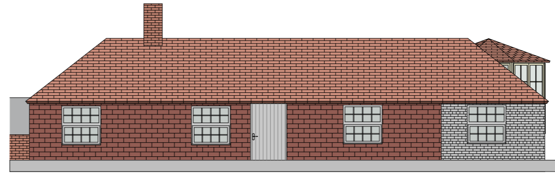
Existing East Elevation 1:100
