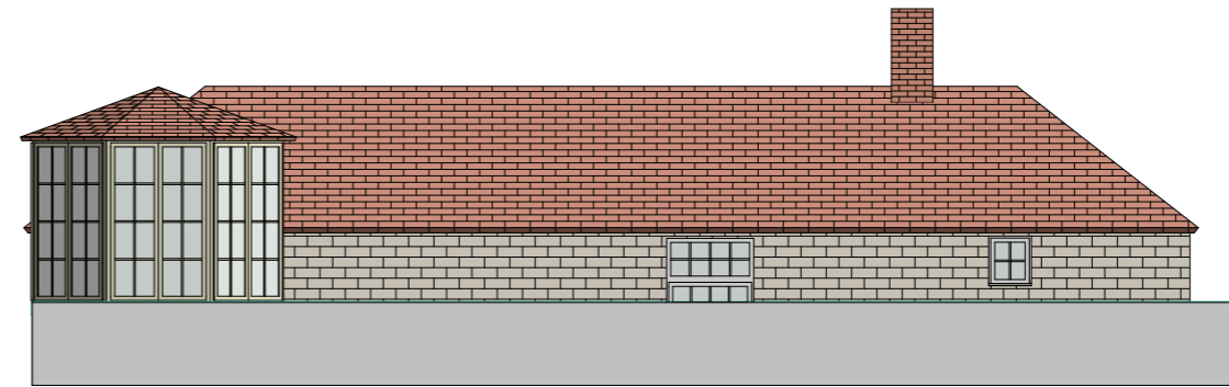
Existing West Elevation 1:100
