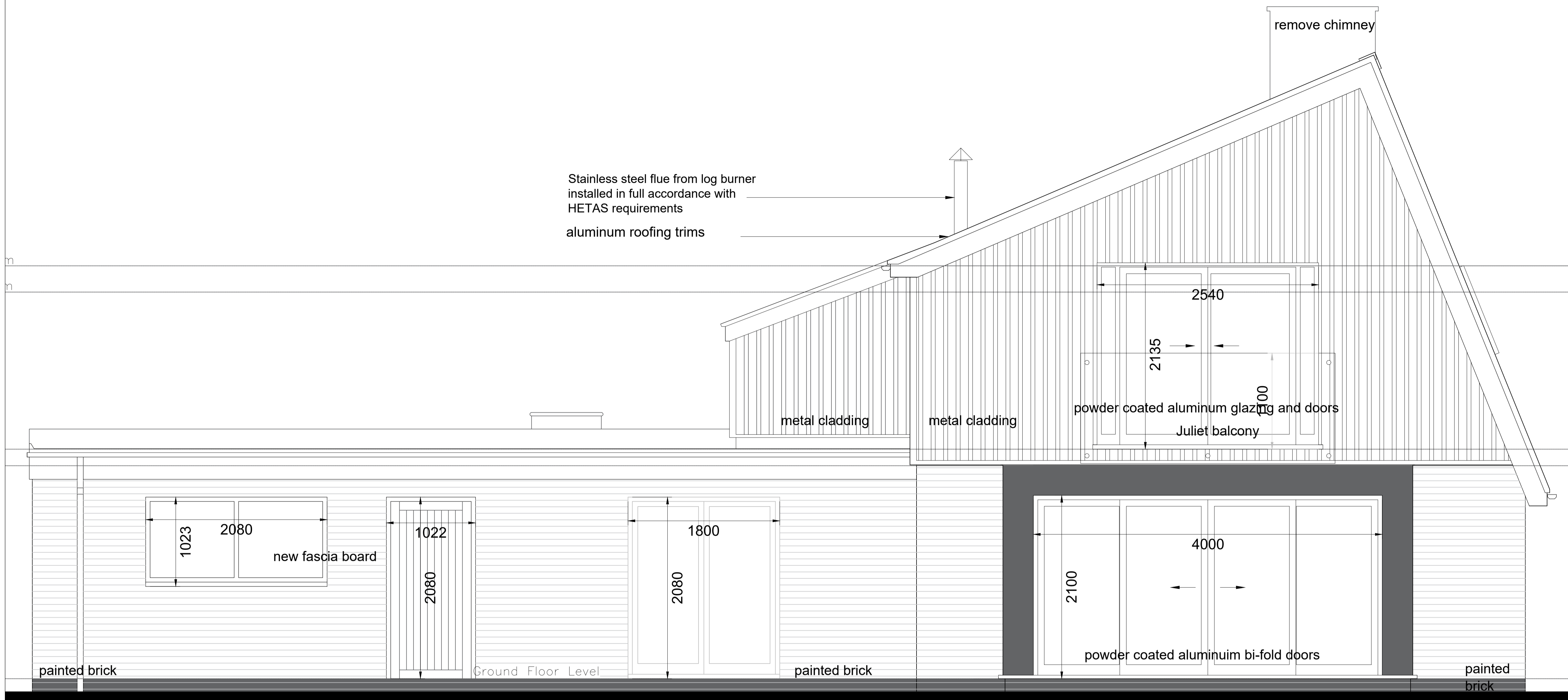
REAR ELEVATION 1:25@A1
