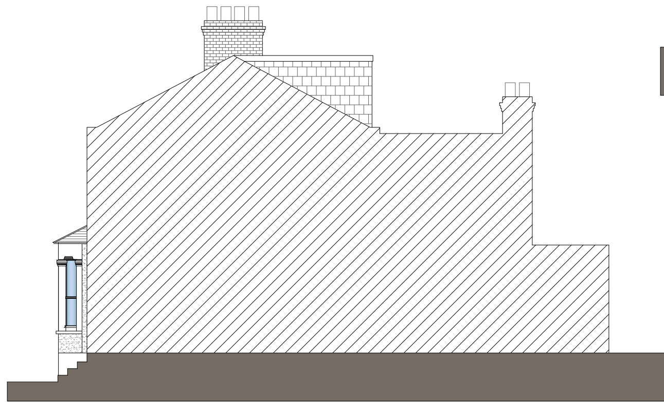
EAST ELEVATION
