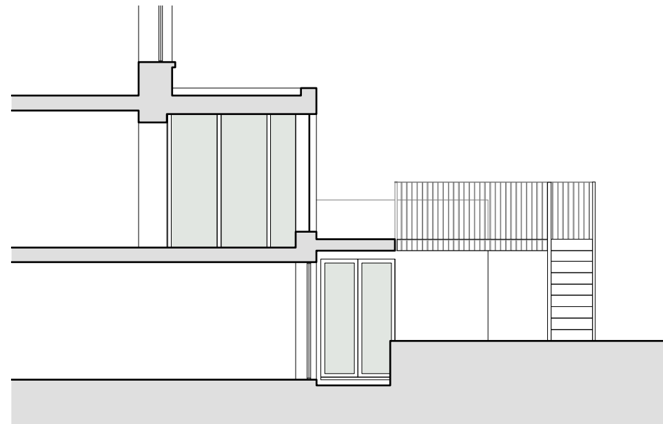
03 Proposed side elevation 1:100 @ A3
