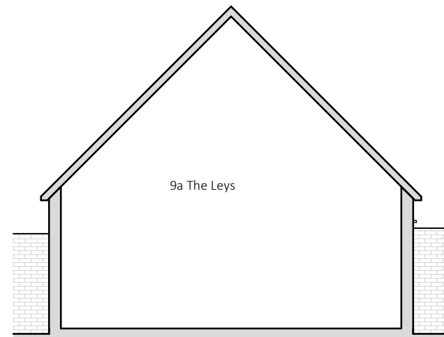
4 p102 08.0 west elevation - existing 1 : 100
