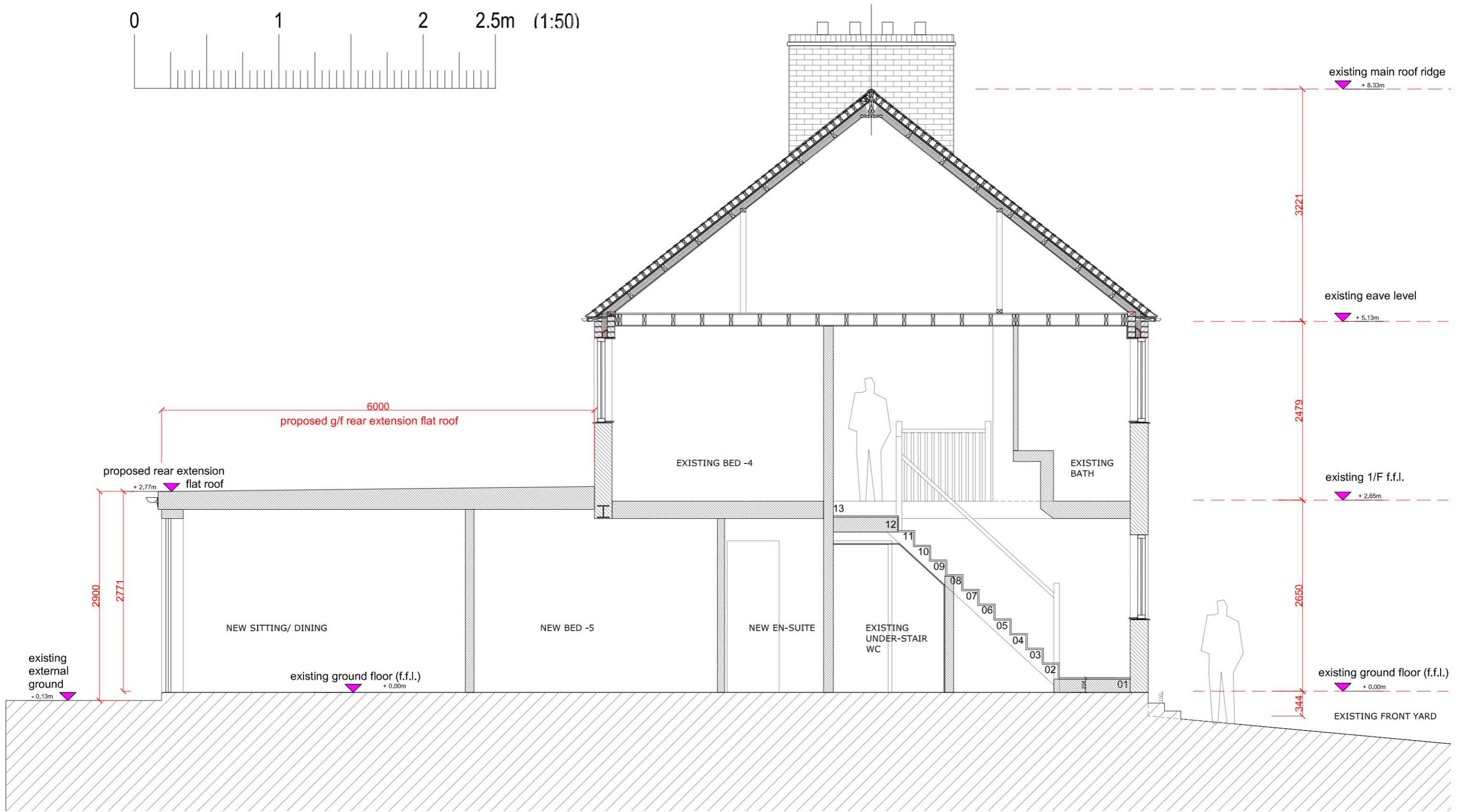
PROPOSED SECTION 1:50
