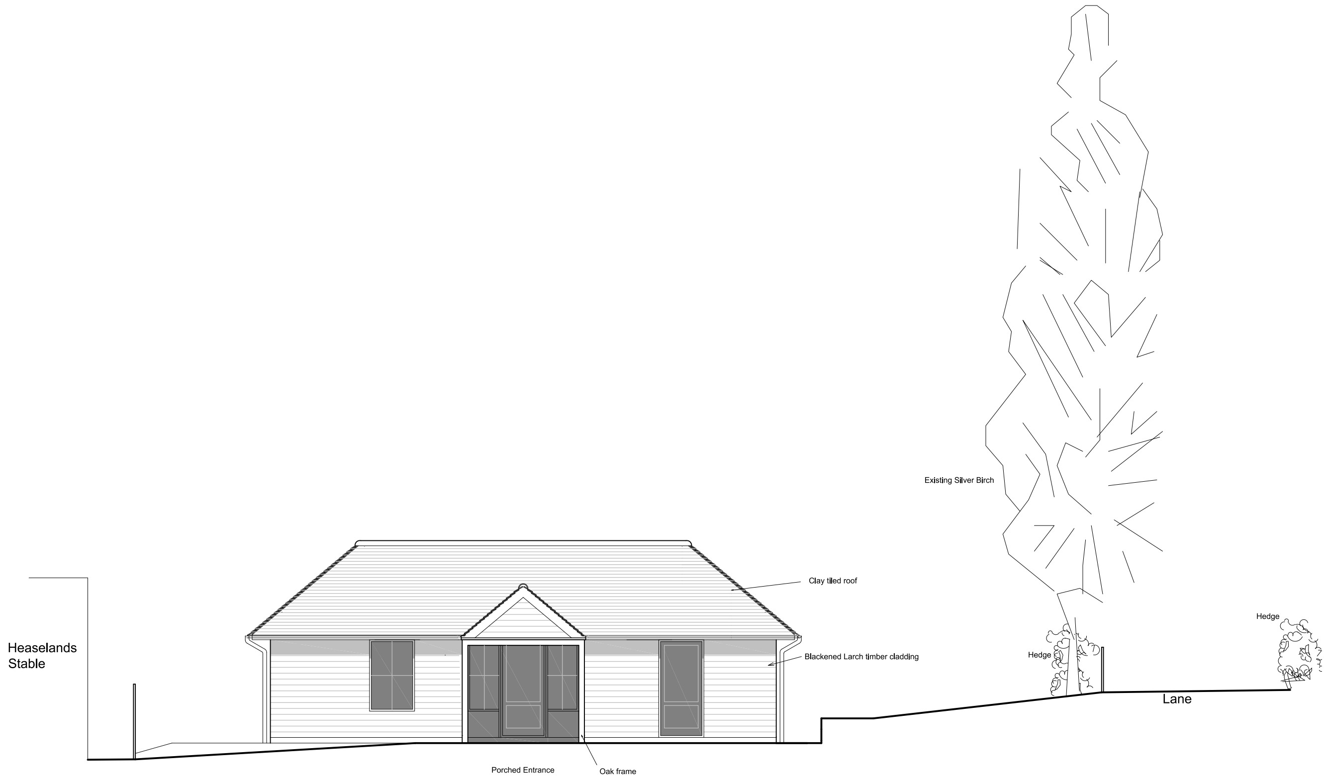
North Elevation
