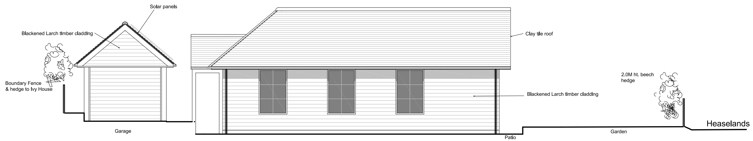
West Elevation
