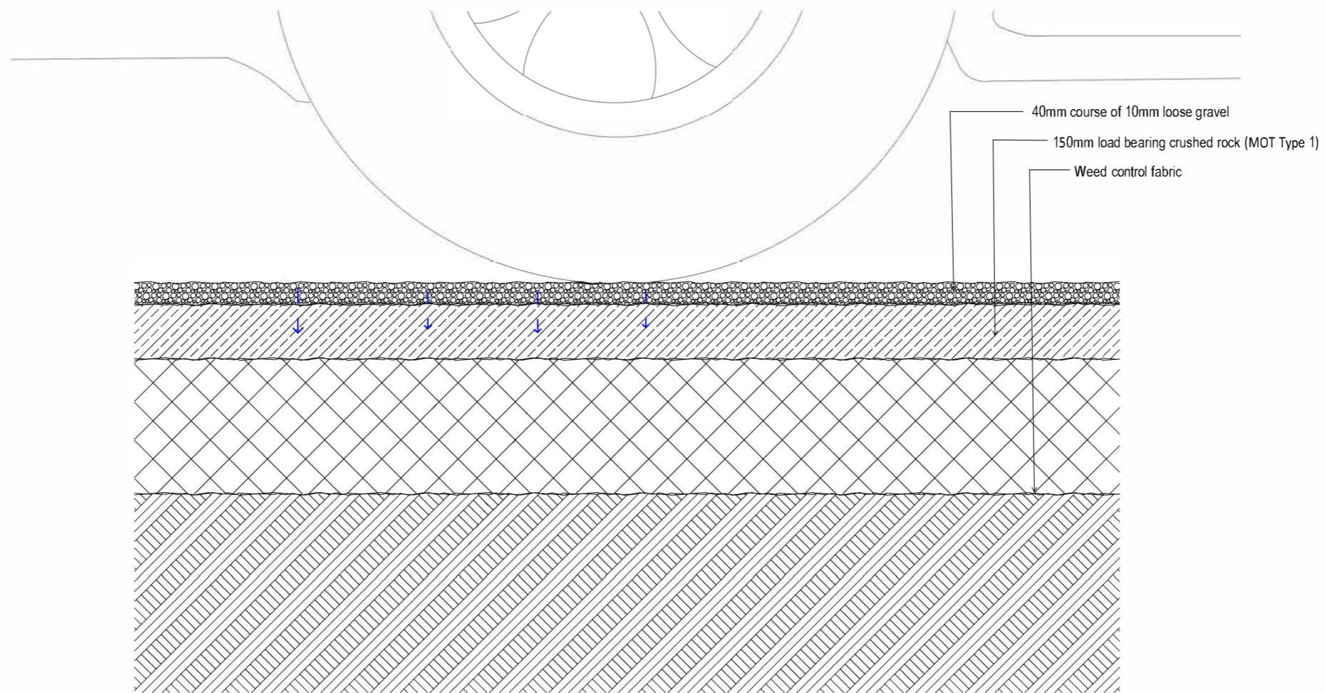
Typical section through unbound gravel surface
