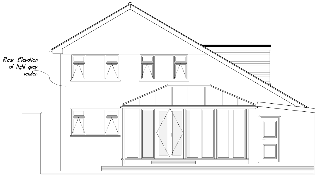
EXISTING REAR (SOUTH) ELEVATION 1:100
