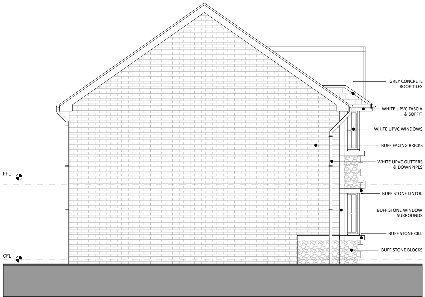
NORTH ELEVATION
