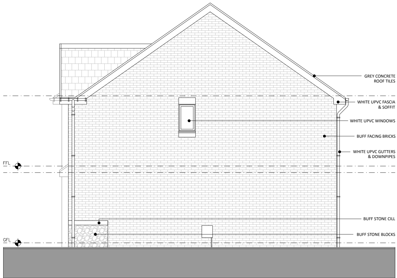
SOUTH ELEVATION
