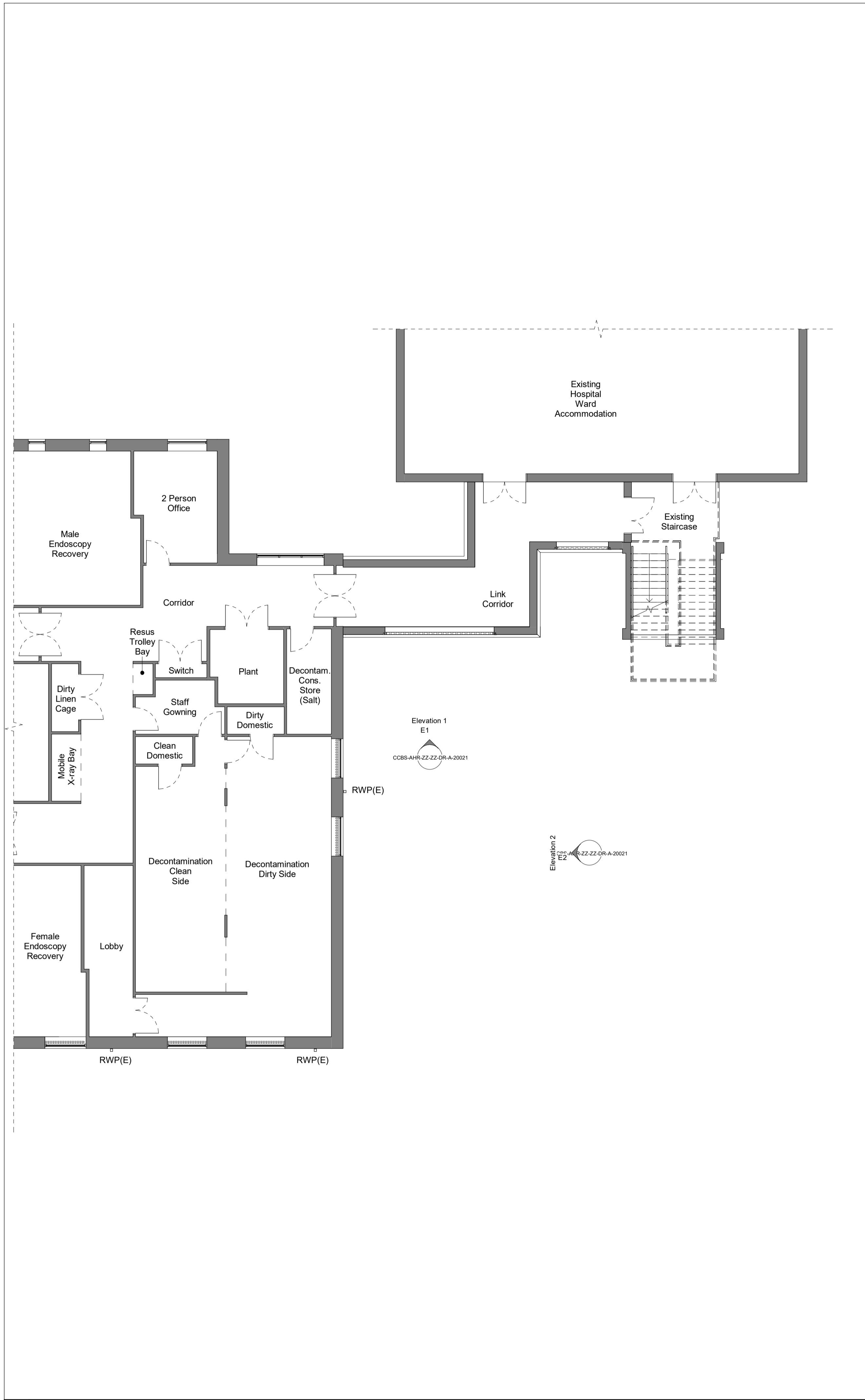
1 Ground Floor GA Plan - Existing 1:100
