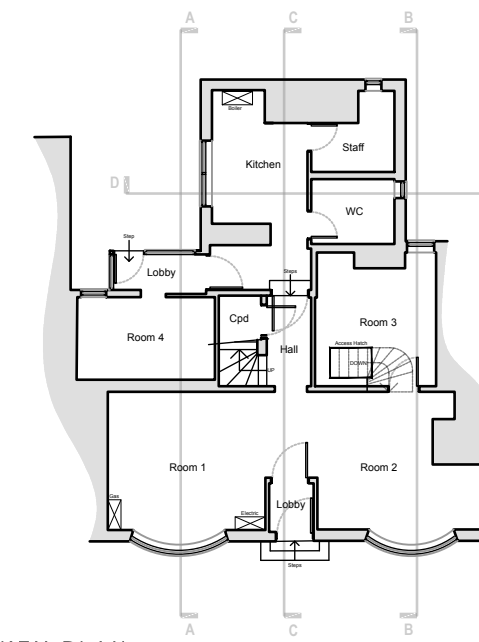
KEY PLAN
