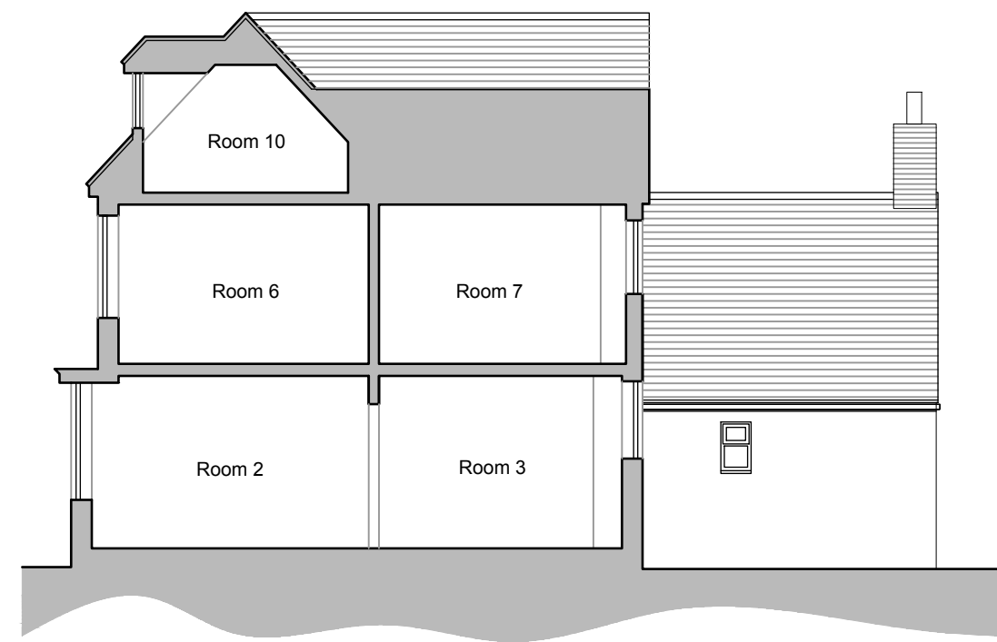
SECTION BB & PARTIAL SIDE ELEVATION
