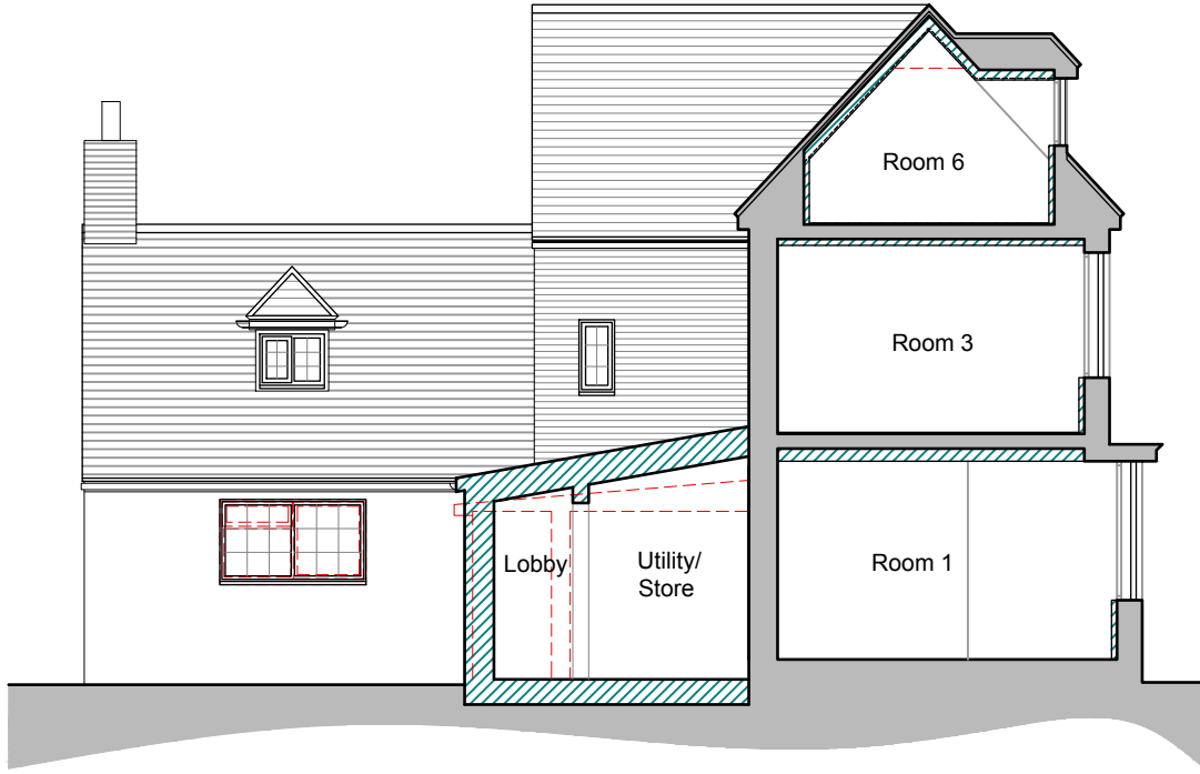
SECTION AA & PART SIDE ELEVATION
