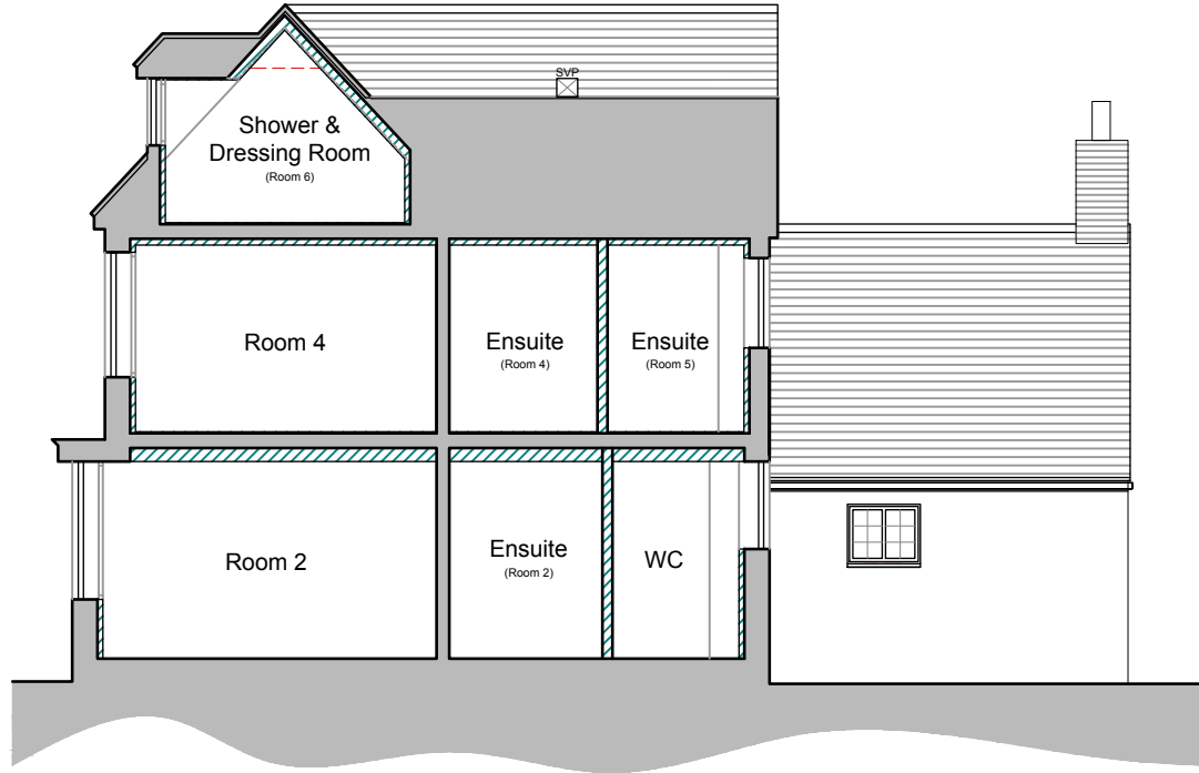
SECTION BB & PARTIAL SIDE ELEVATION
