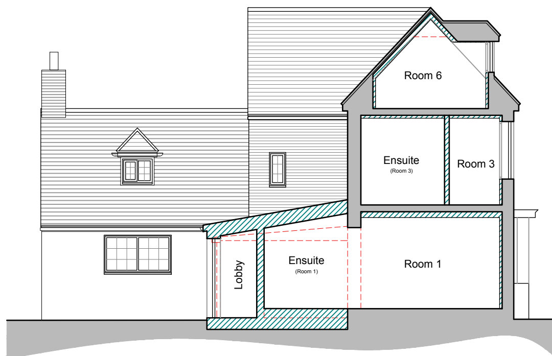
SECTION EE
