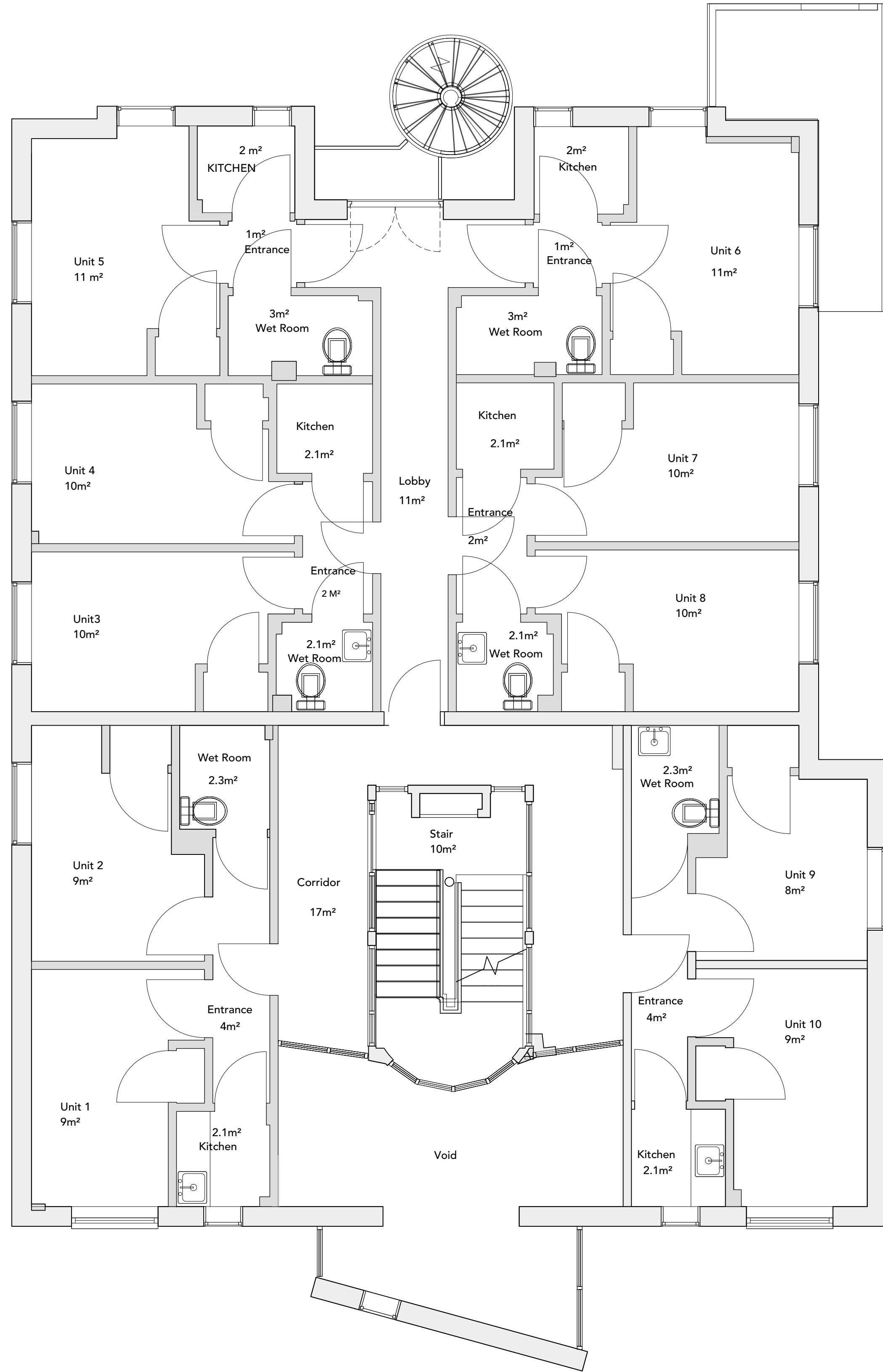
First Floor - Existing 1:50 @ A1
