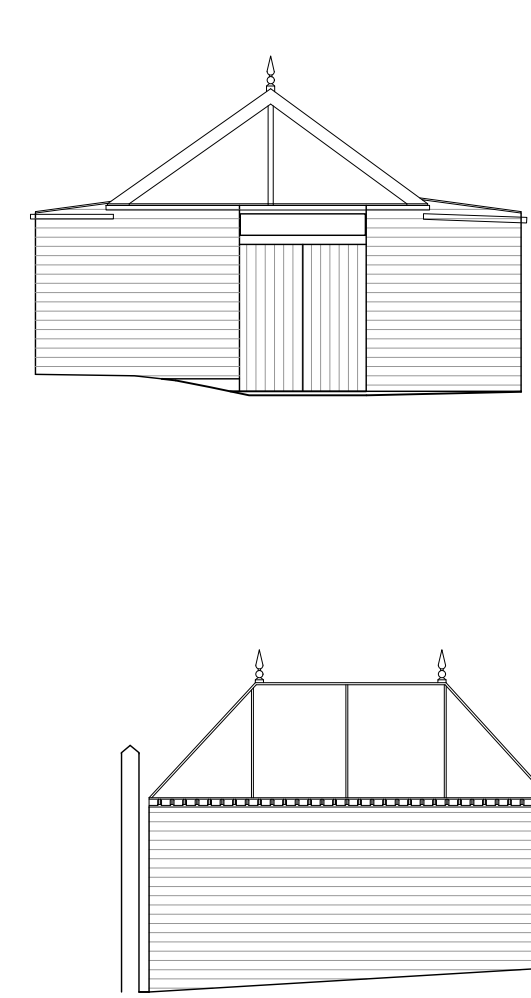
East Elevation 1:100
