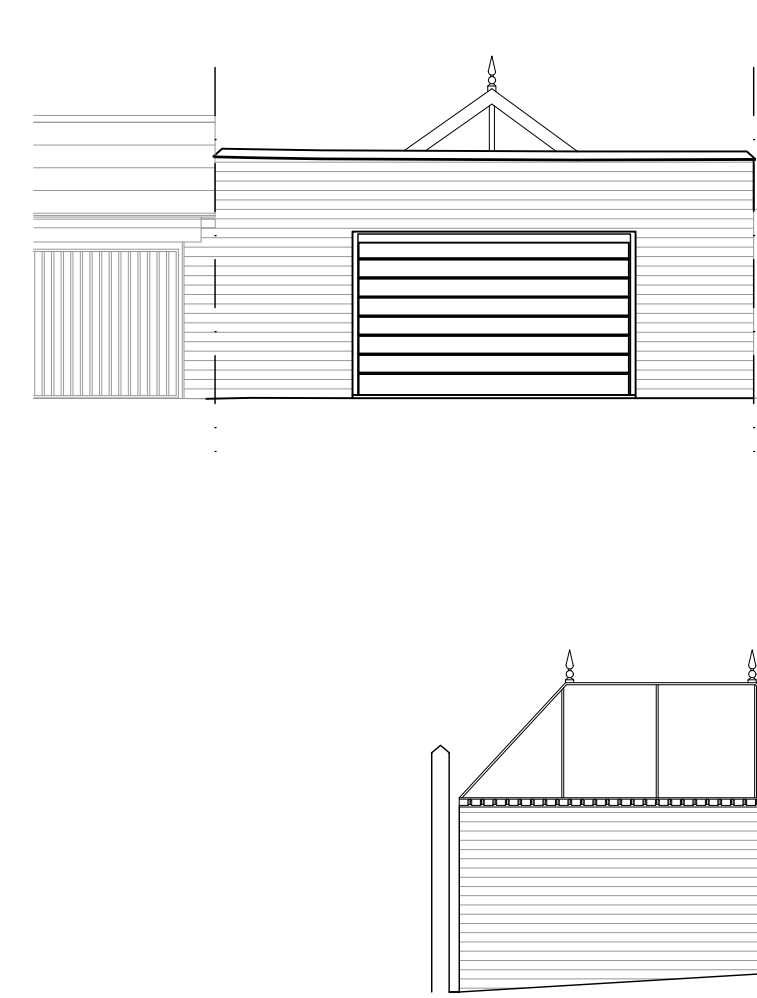
East Elevation 1:100
