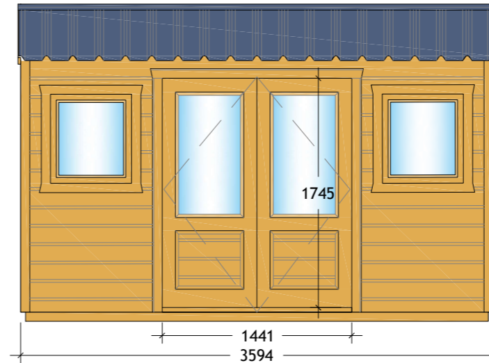
FRONT ELEVATION
