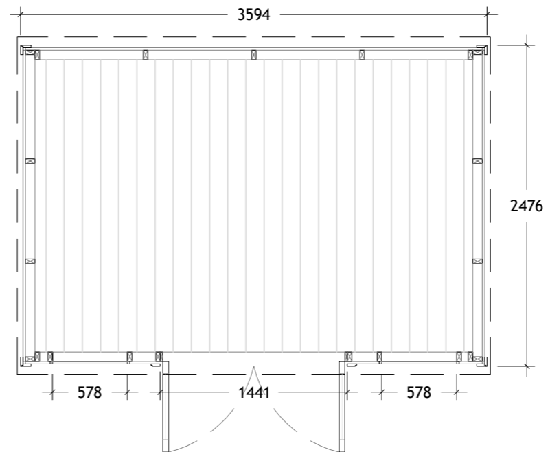
VIEW PLAN
