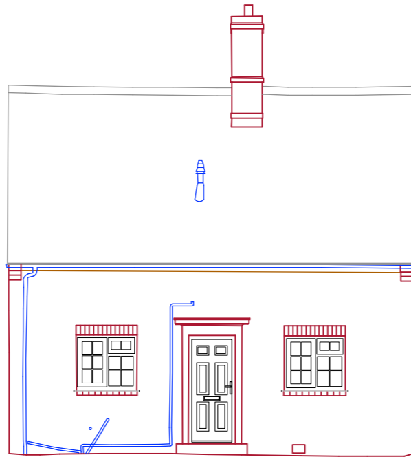
North Elevation
