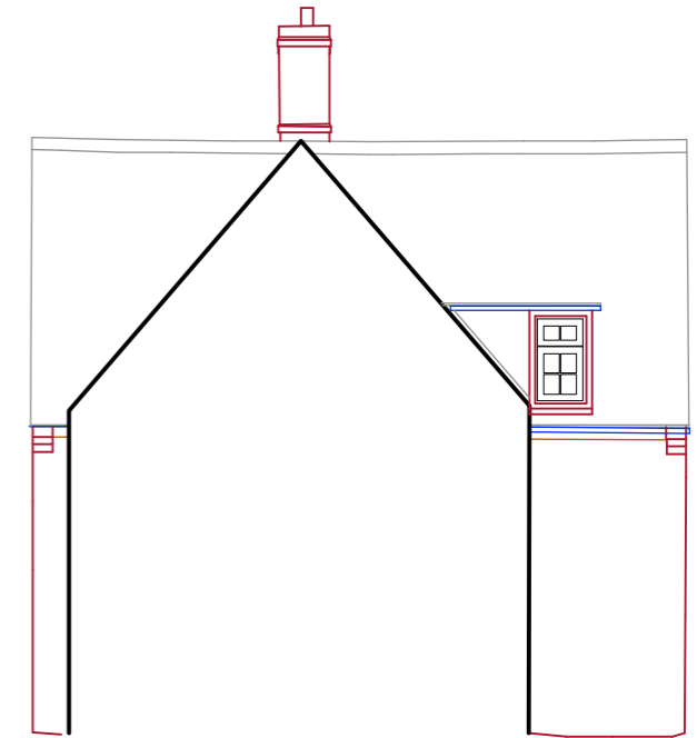
South Elevation
