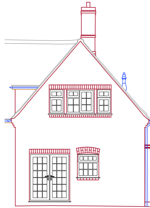
East Elevation
