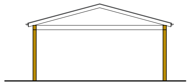
PROPOSED SECTION 1:100 SCALE
