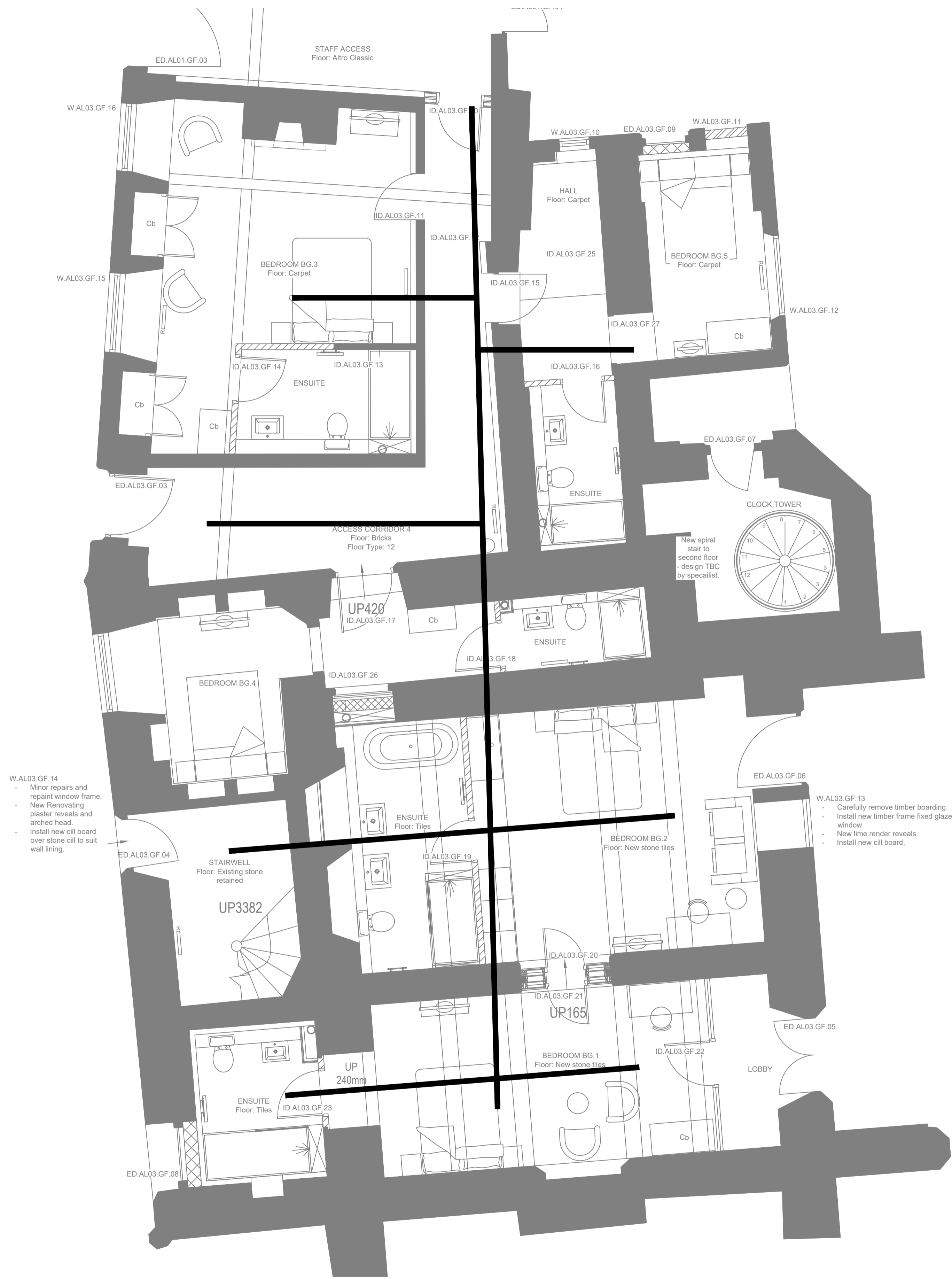
GROUND FLOOR (1:50@A1)
