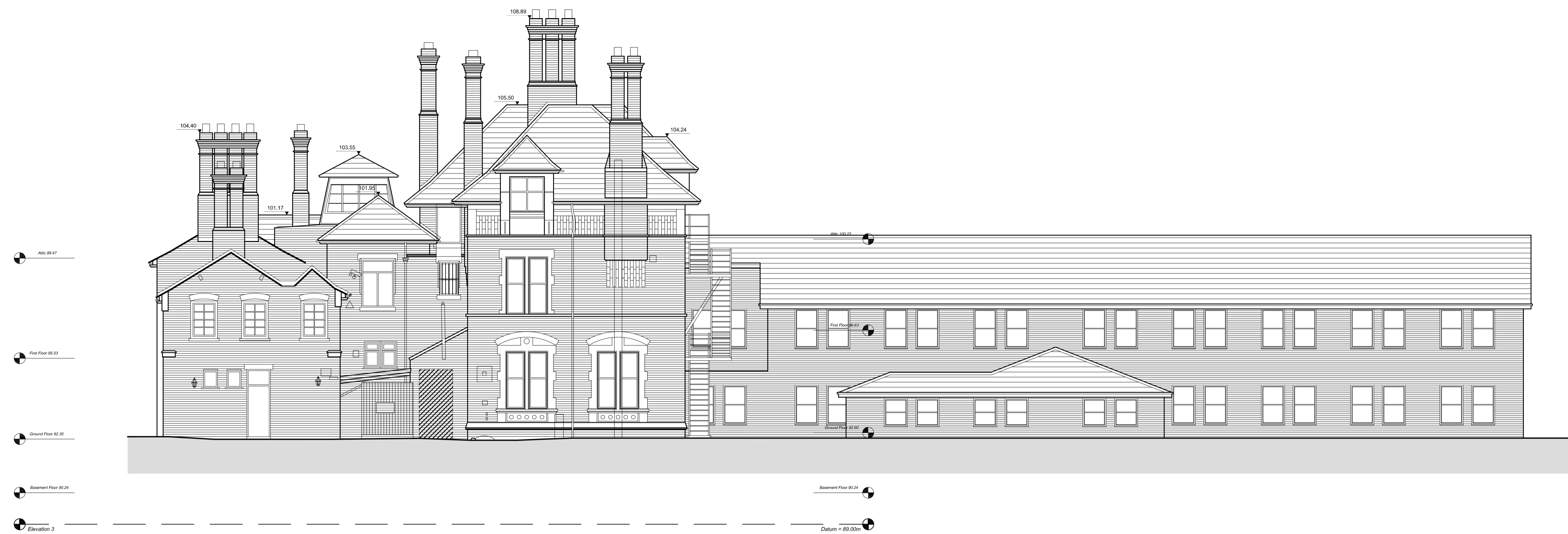
EXISTING NORTH ELEVATION 1:100
