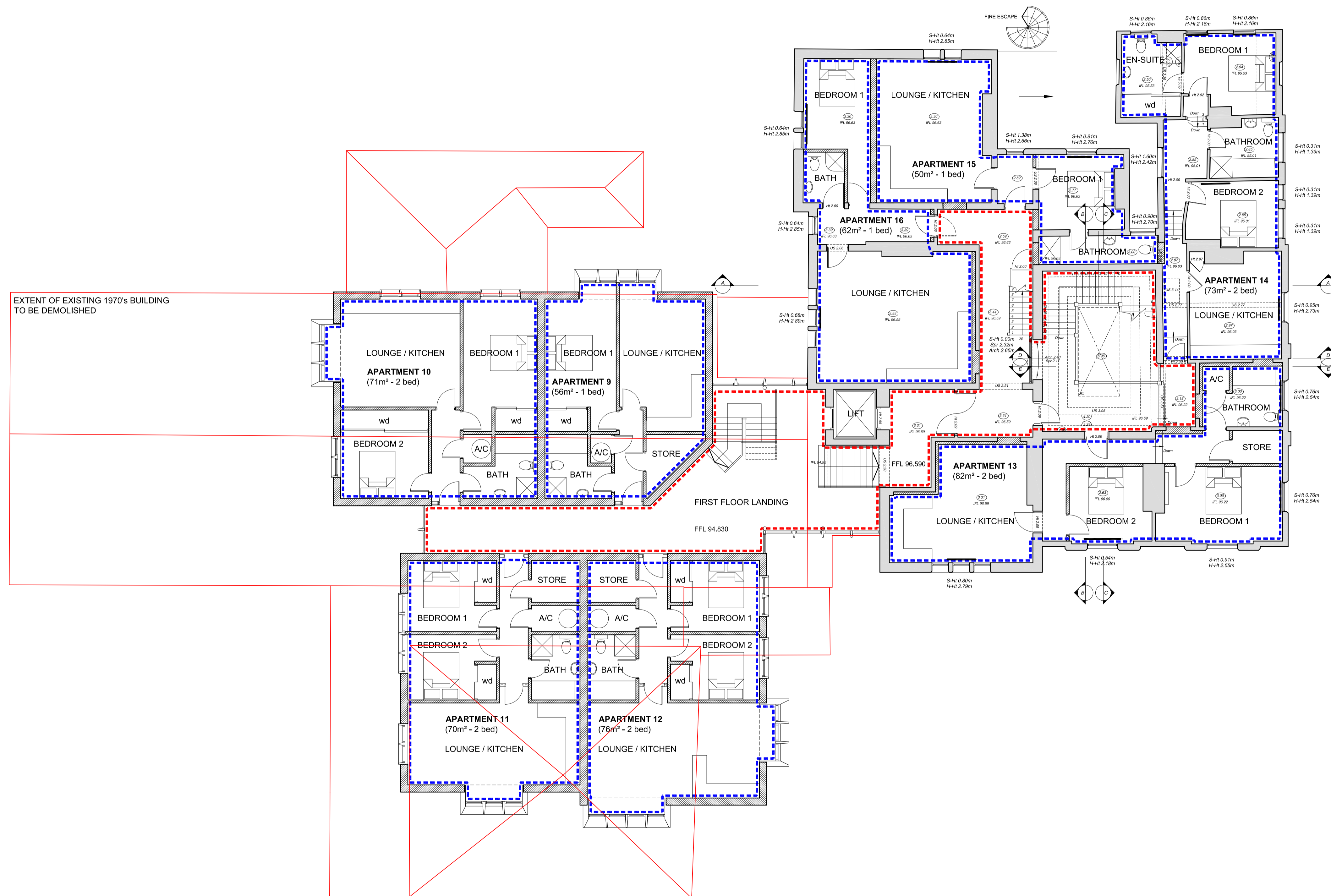
PROPOSED FIRST FLOOR PLAN 1:100
