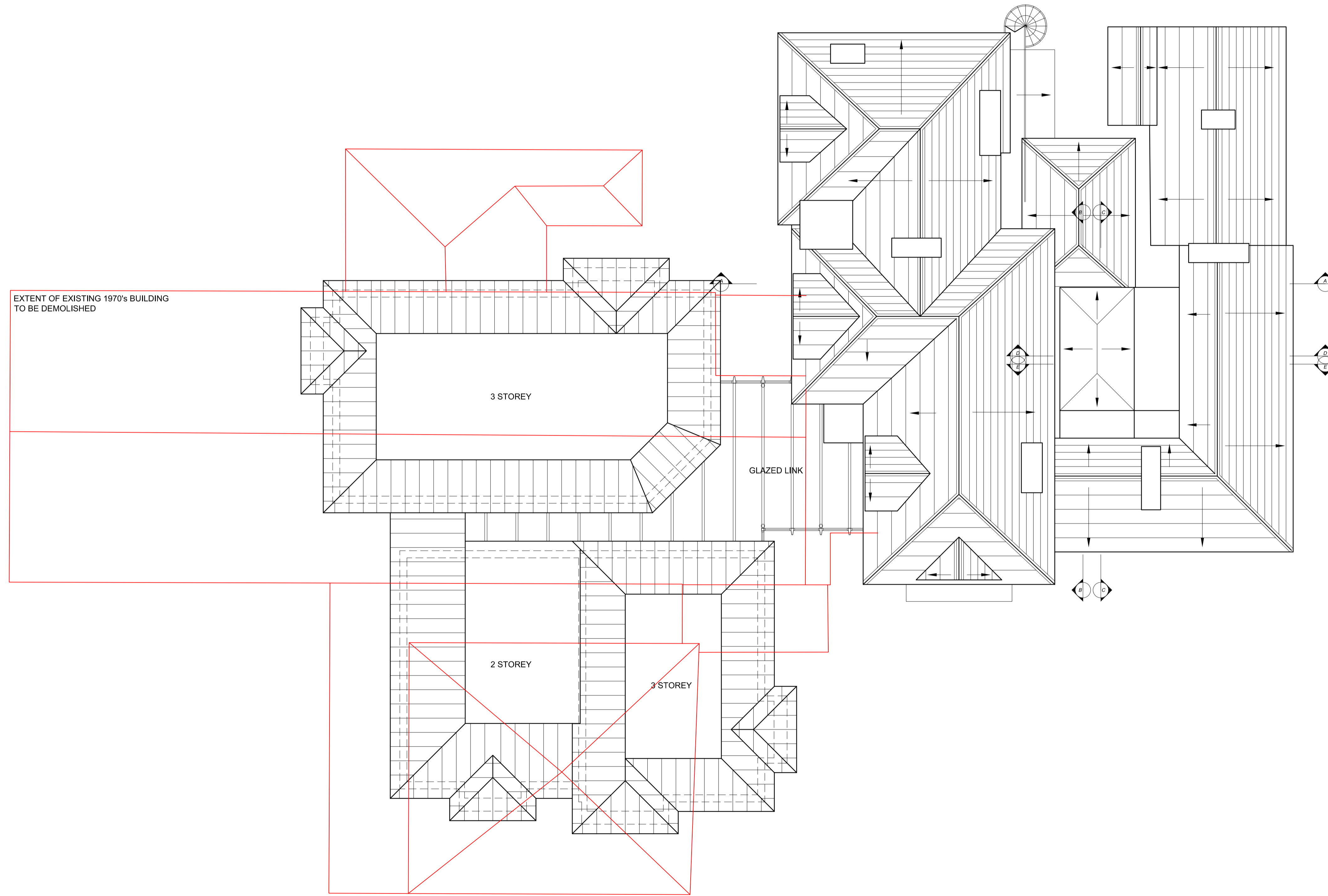
PROPOSED ROOF PLAN 1:100
