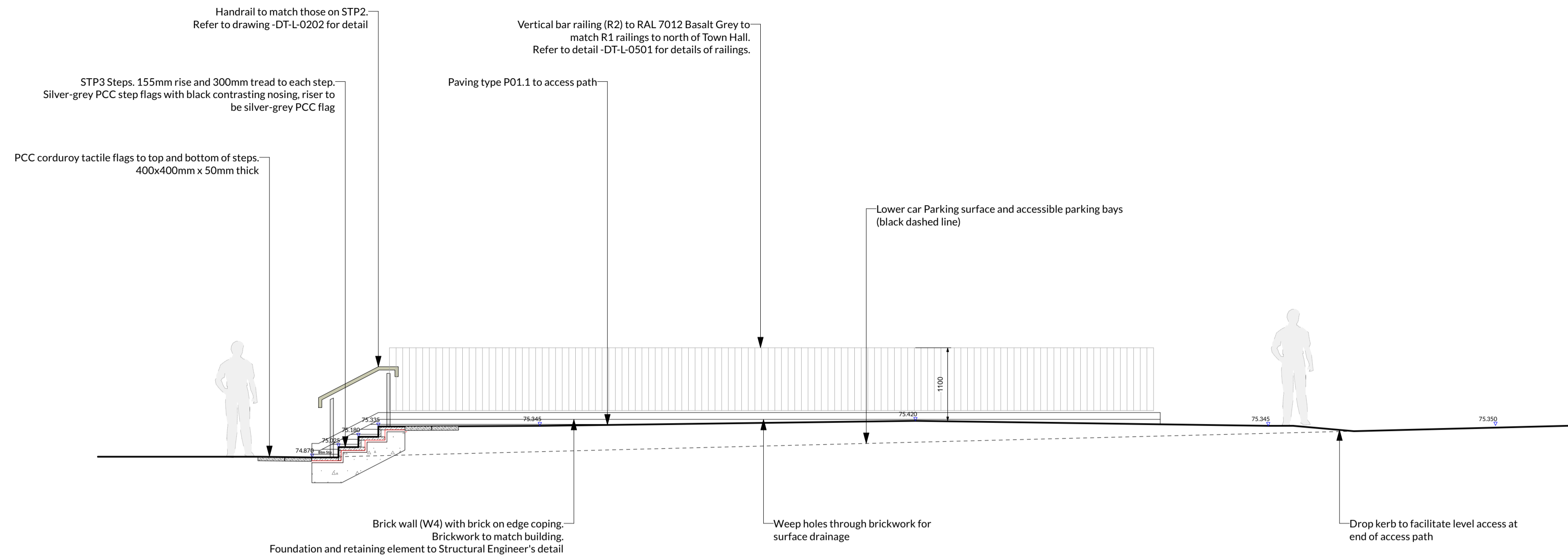
Long Section Through Access Path and Retaining Walls Scale 1:50 @ A1
