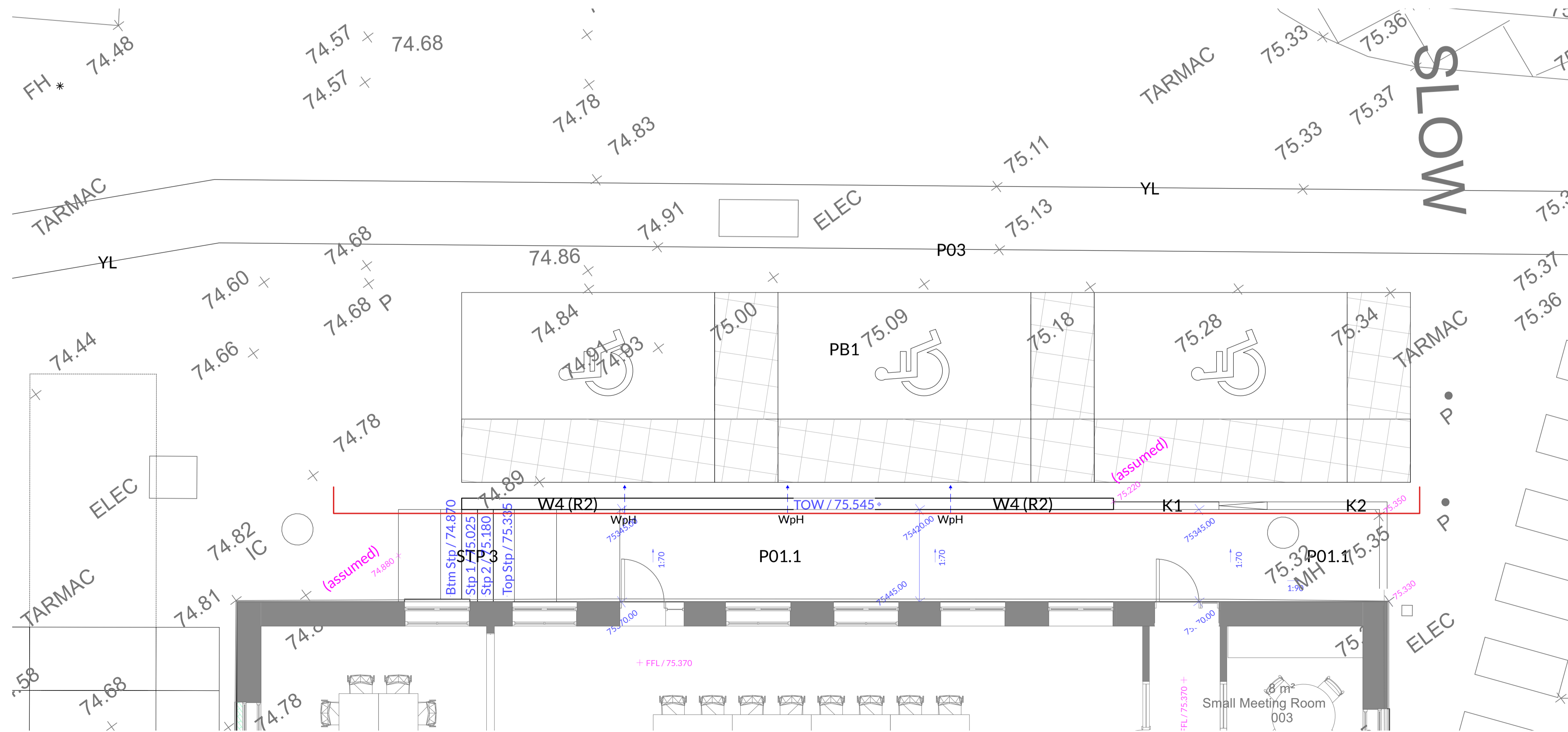
Plan View of Access Path and Retaining Walls Scale 1:50 @ A1
