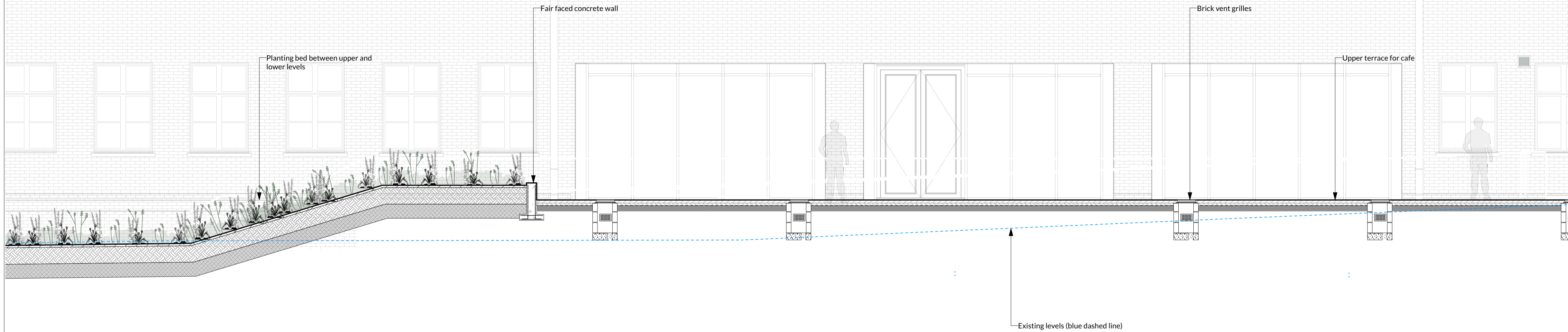
Long Section Through Cafe Terrace (Interface With Building) Scale 1:50 @ A1
