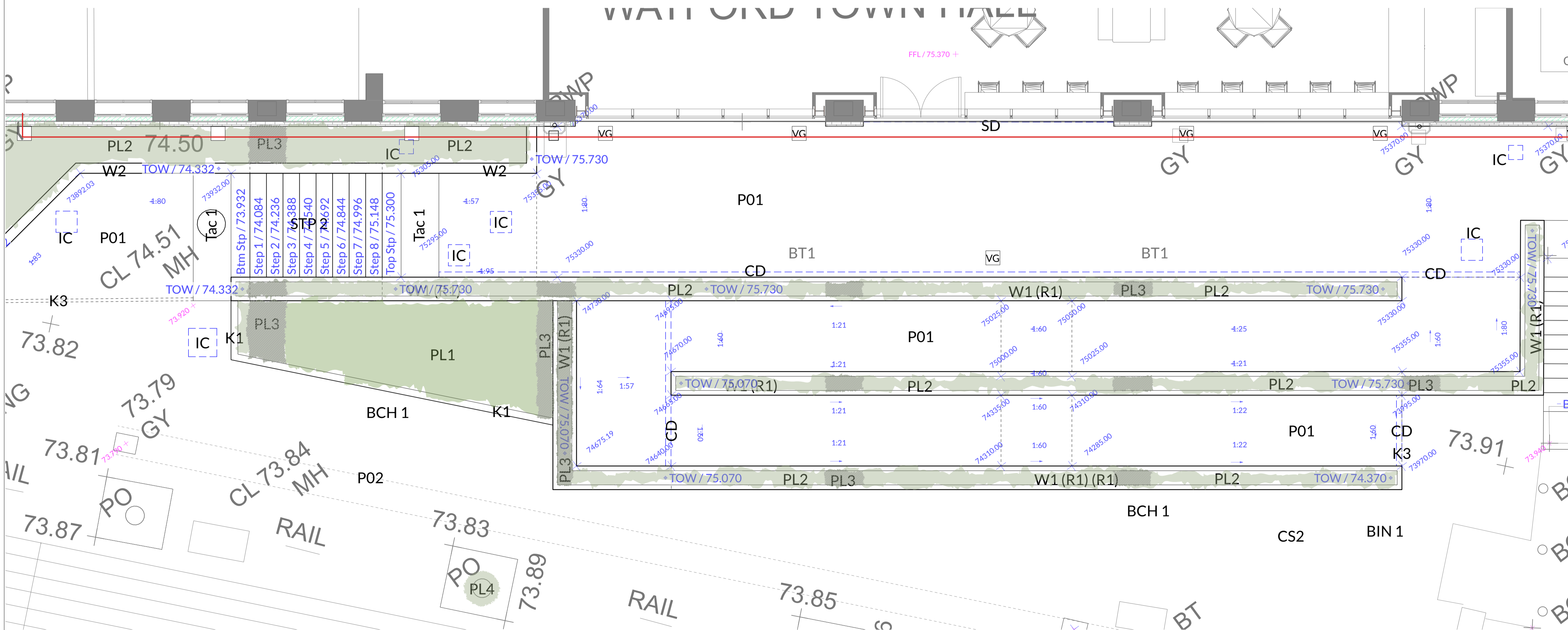
Plan View of Cafe Terrace (Interface With Building) Scale 1:50 @ A1
