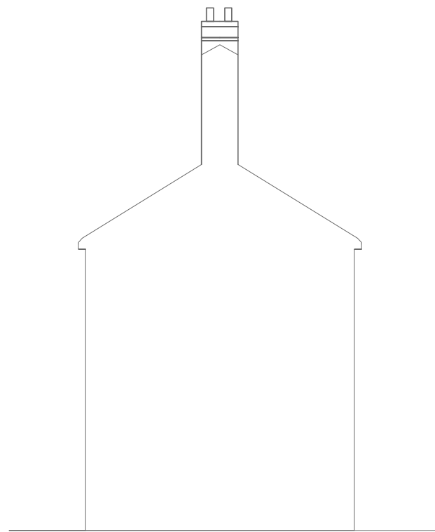
Proposed west elevation 1:100
