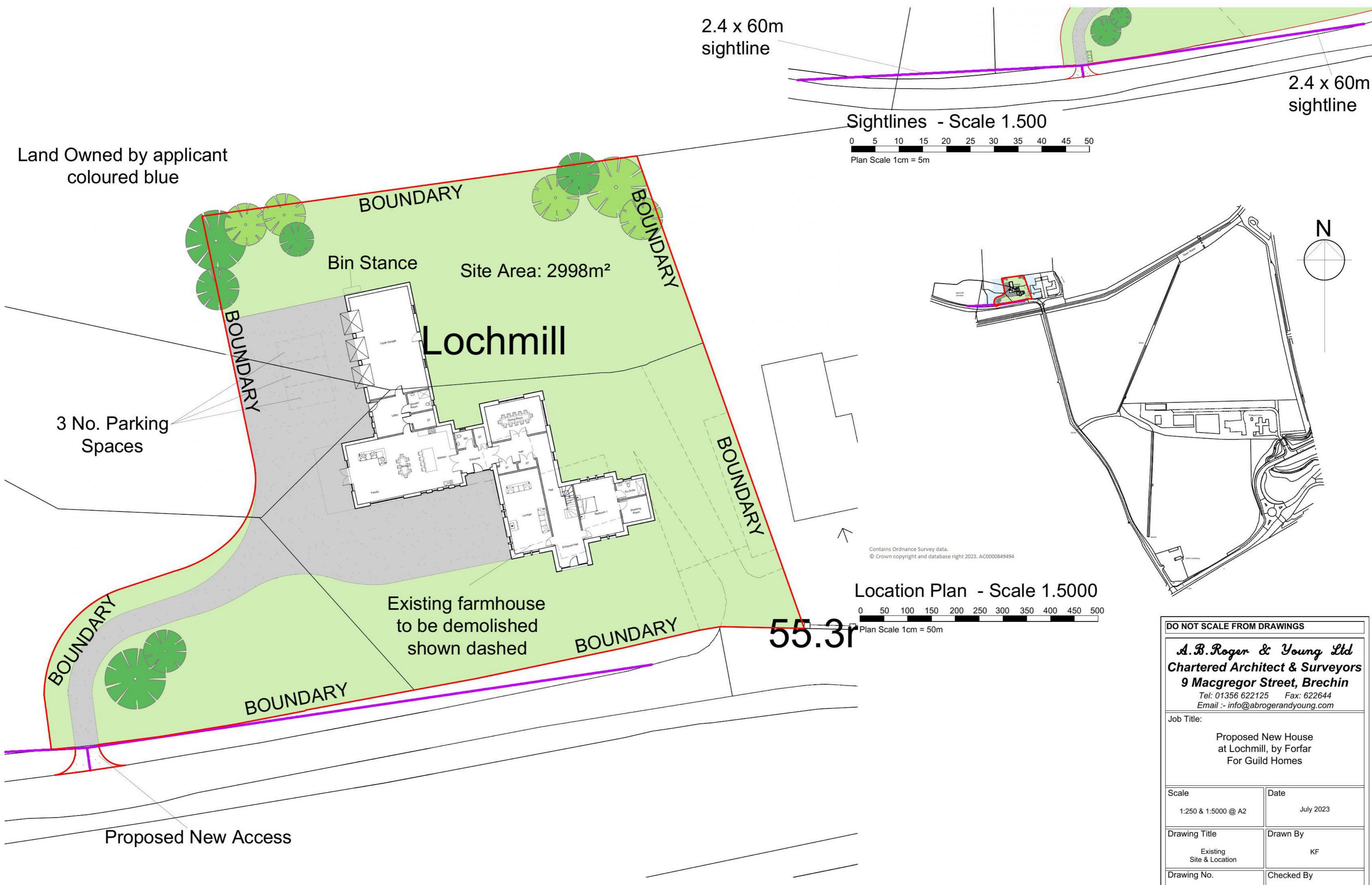
Site Plan - Scale 1.250
