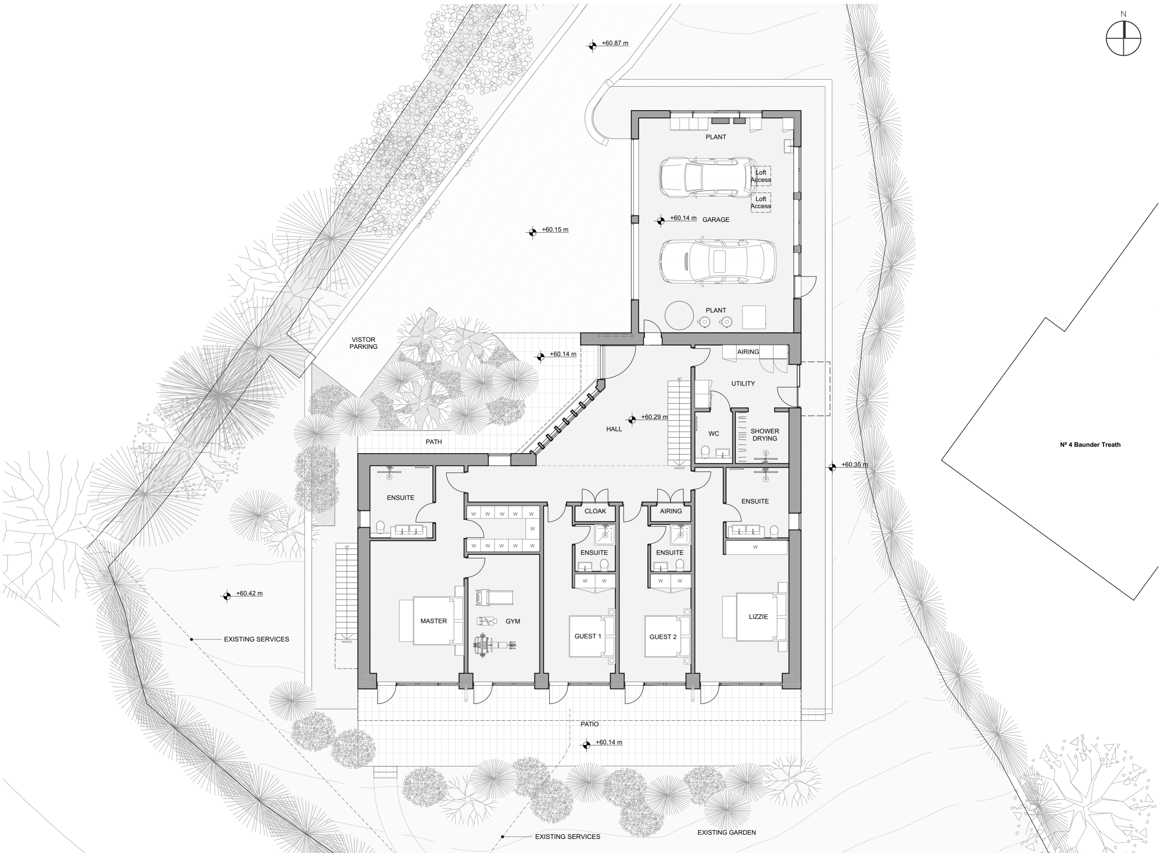
GF-GROUND FLOOR PLAN 1:100
