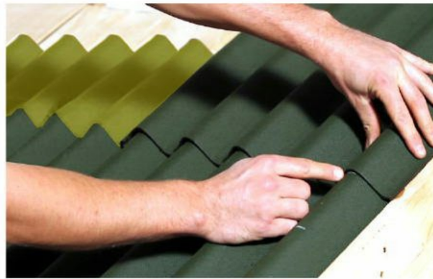
1 corrugation lap
