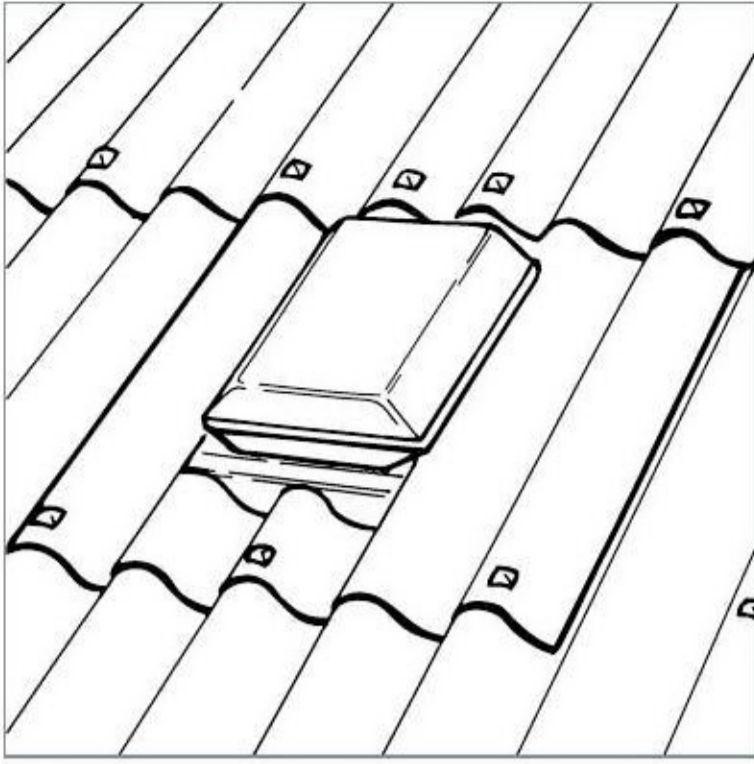
Onduline roof ventilators For assured roof ventilation.
