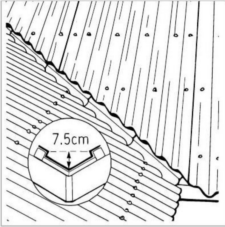
Onduline valley detail Minimum 7.5 cm valley drainage
