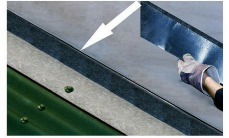
Upstand to wall To allow for differential movement between the wall and the roof sections always use a separate wall cover flashing dressed into a prepared joint.
