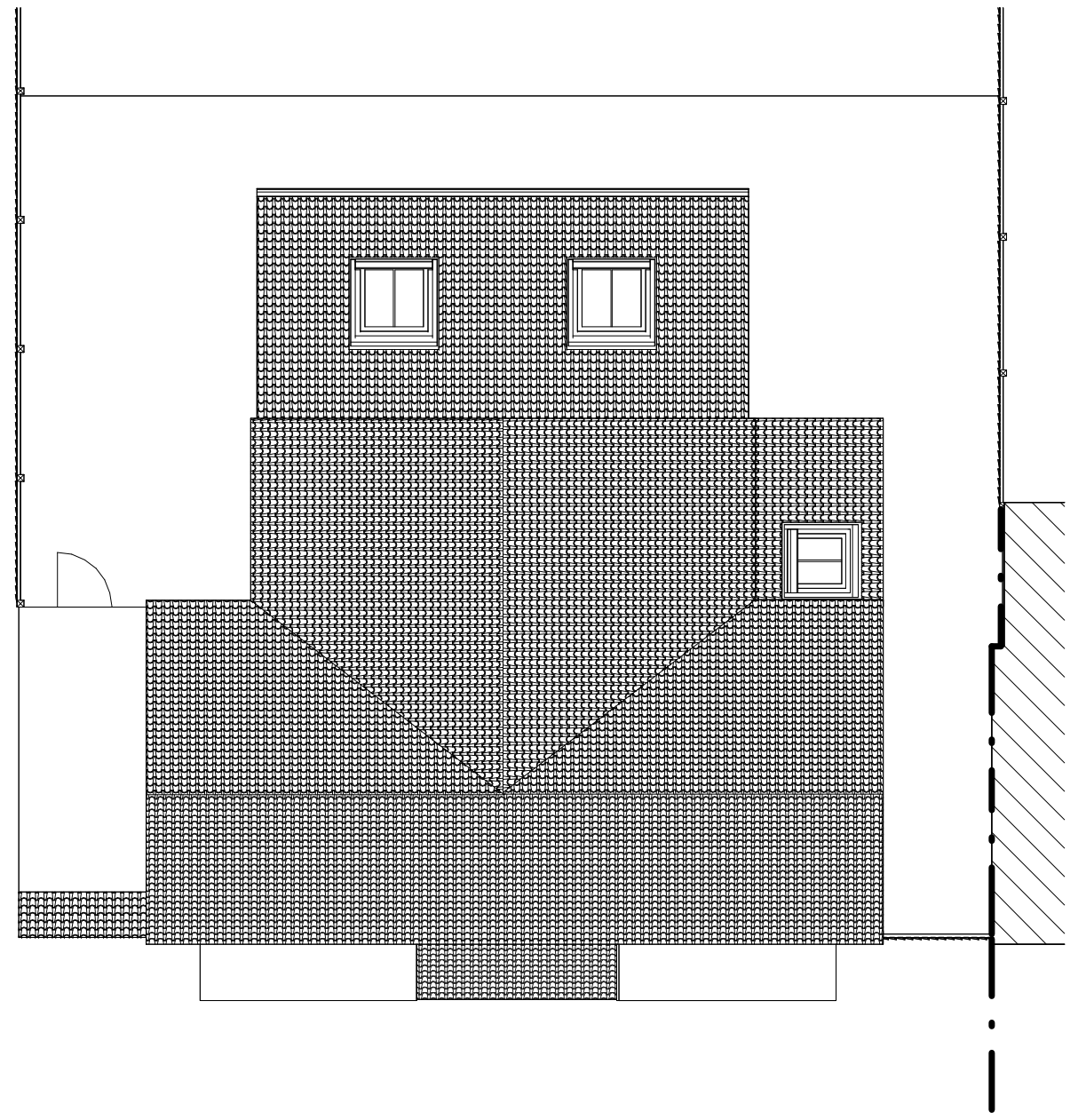
2 Proposed Roof Plan. 1 : 100
