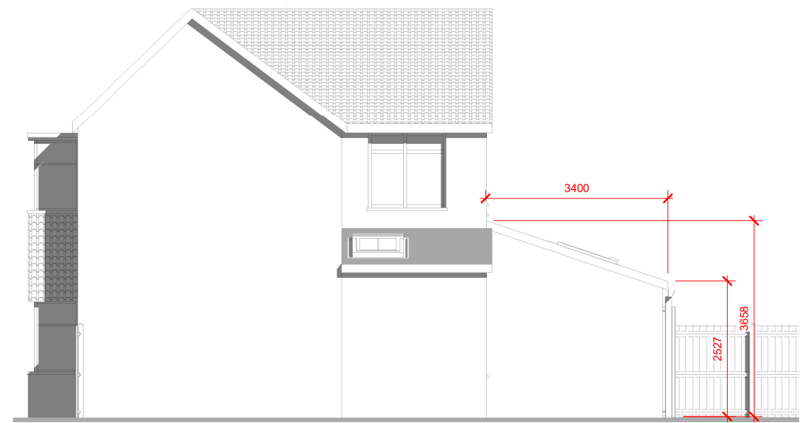
Proposal I Side Elevation II.
