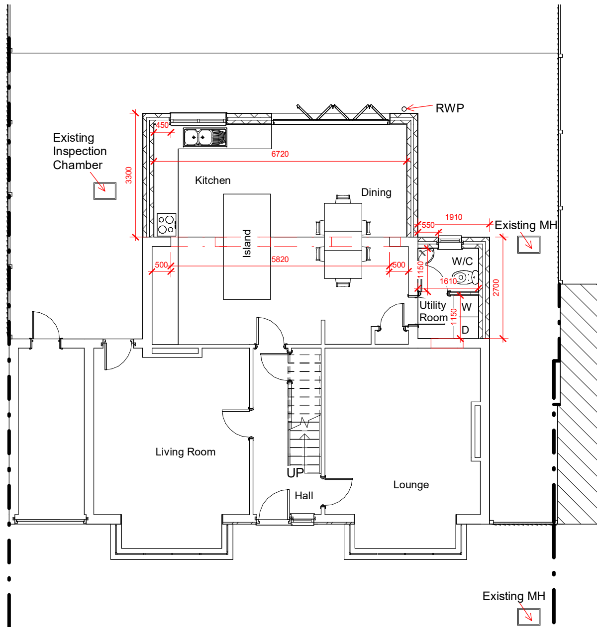
1 Proposed Ground Floor. 1 : 100
