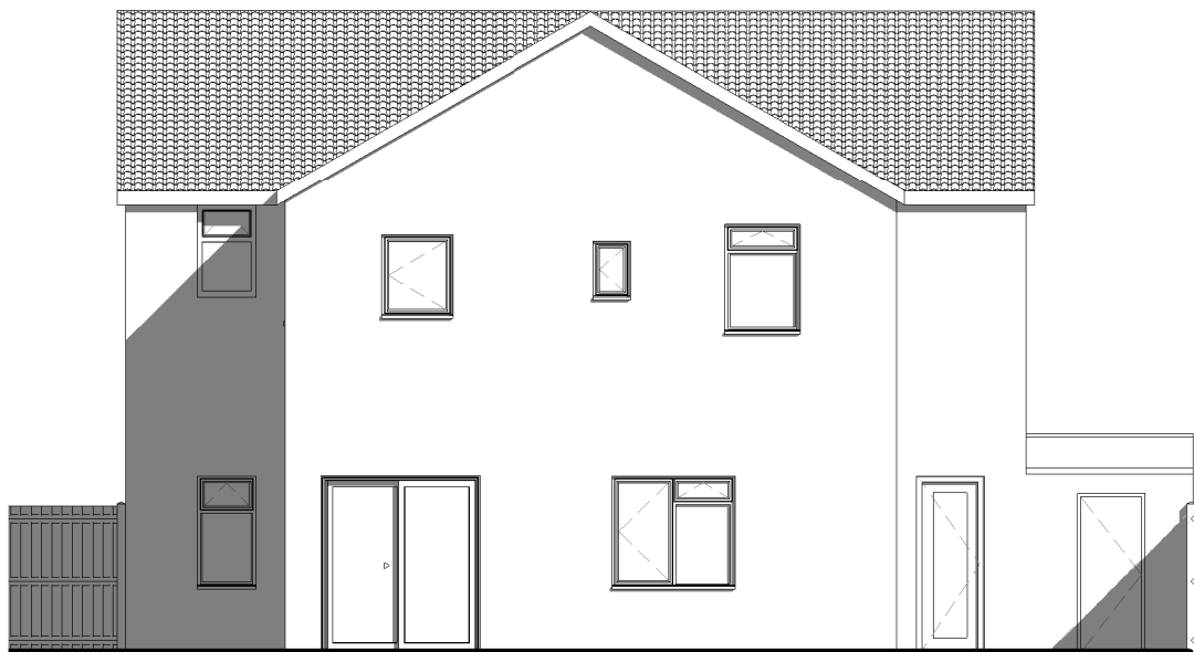
2 Existing Rear Elevation. 1 : 100
