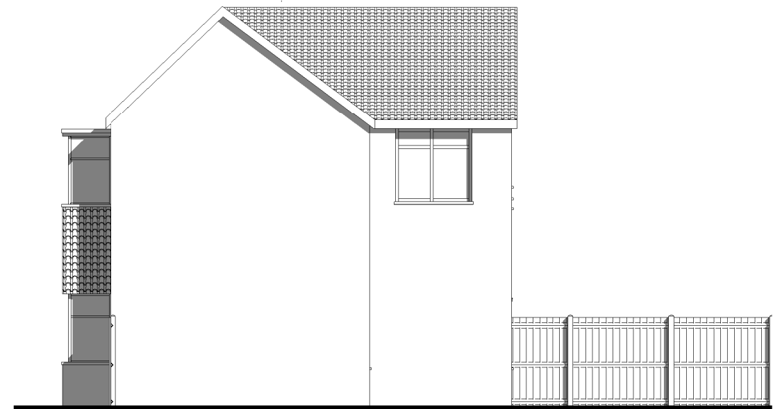
4 Existing Side Elevation II. 1 : 100
