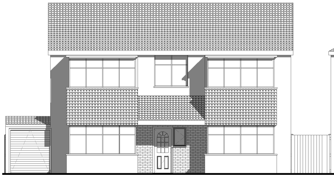
1 Existing Front Elevation. 1 : 100
