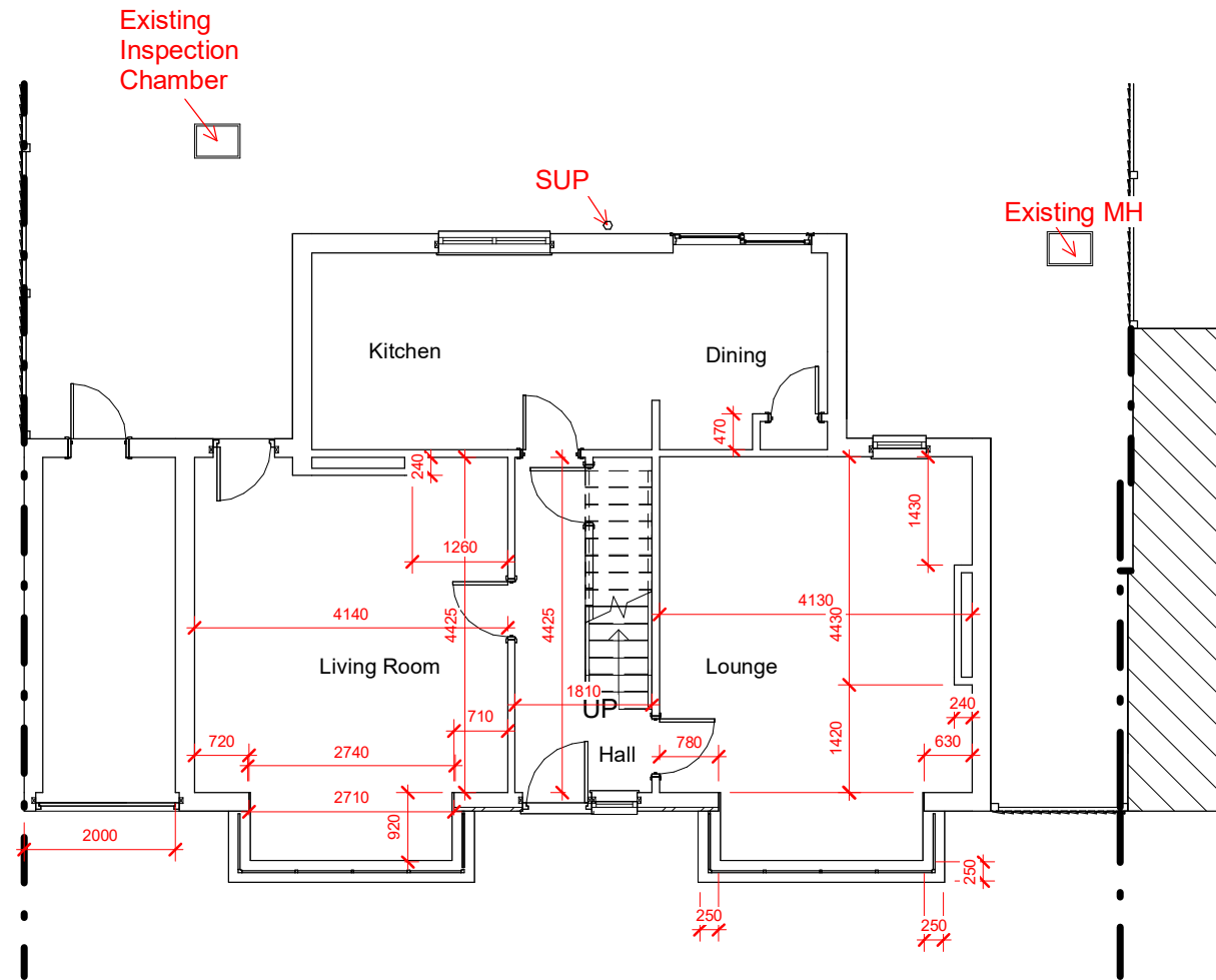
1 Existing Ground Floor. 1 : 100
