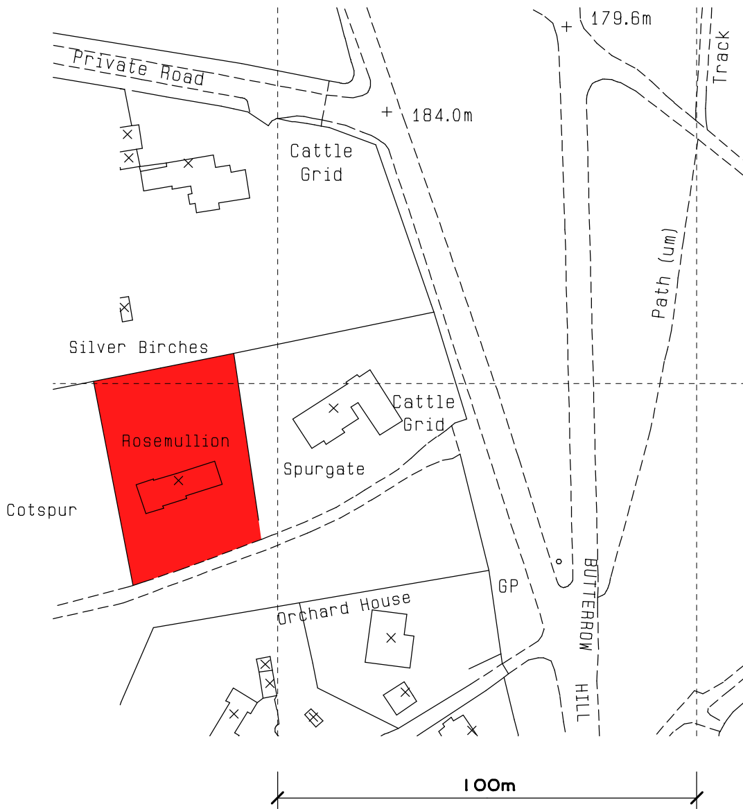
LOCATION PLAN 1:1250
