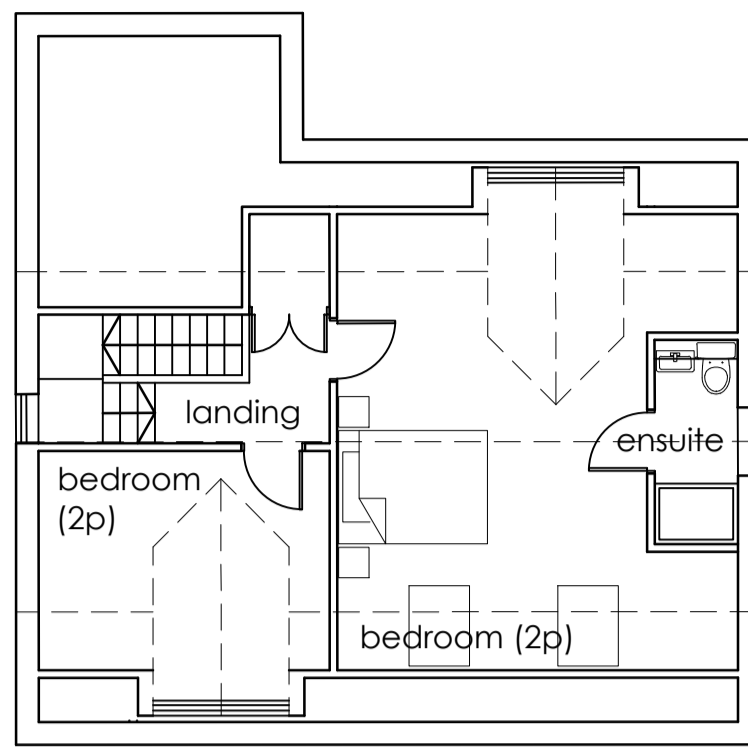
Loft Level Plan (44sqm)
