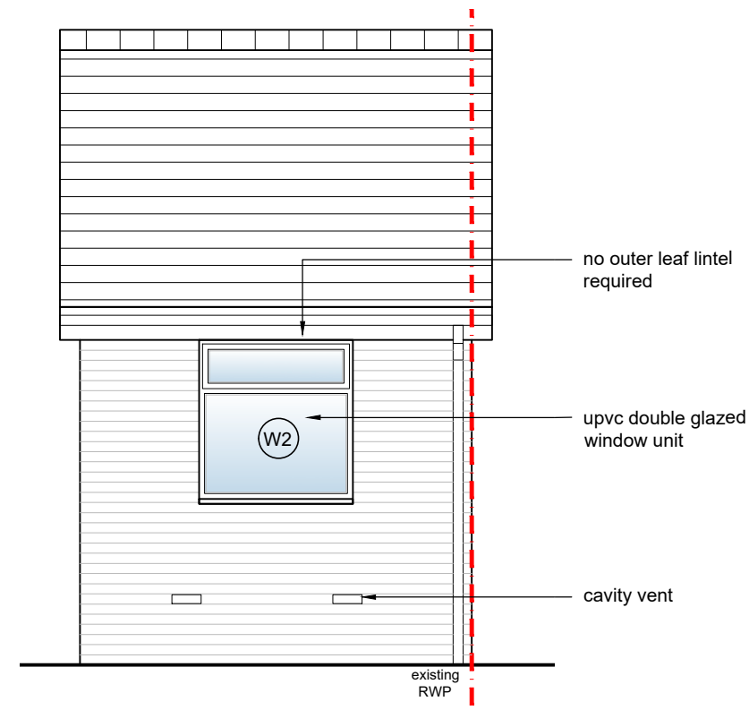
Proposed Rear Elevation 1:50 @ A3
