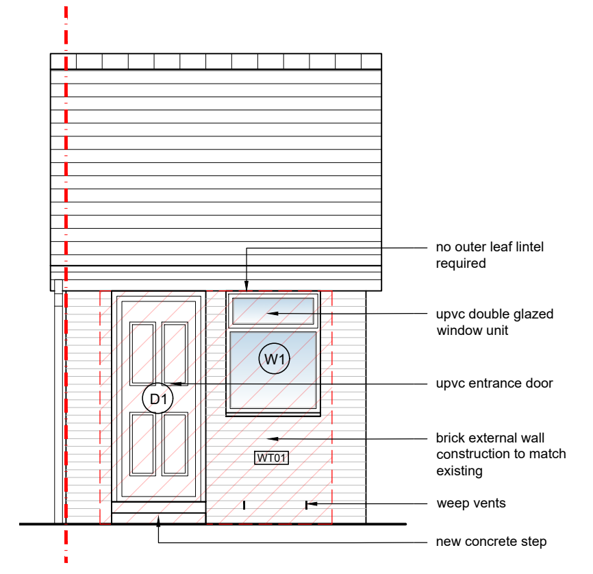
Proposed Front Elevation 1:50 @ A3
