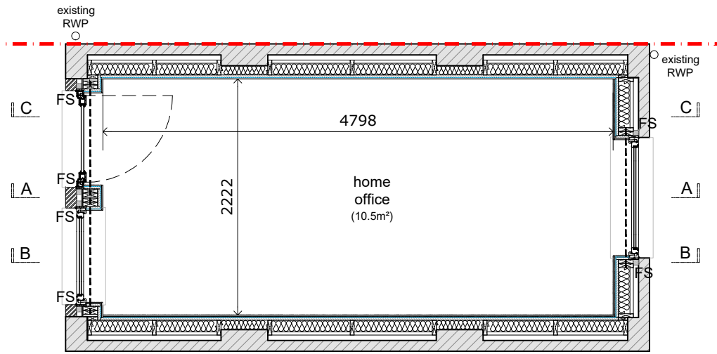
Proposed Floor Plan 1:50 @ A3
