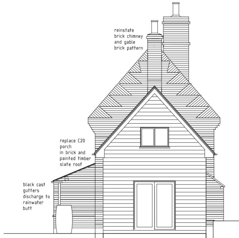
NORTH ELEVATION (REAR GARDEN)
