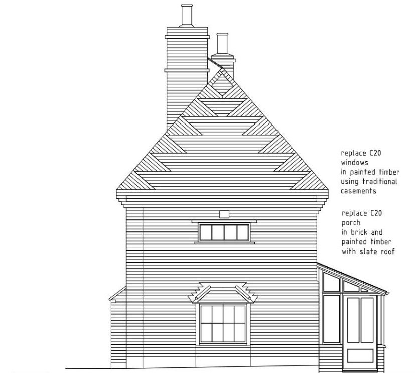
SOUTH ELEVATION (ROADSIDE)
