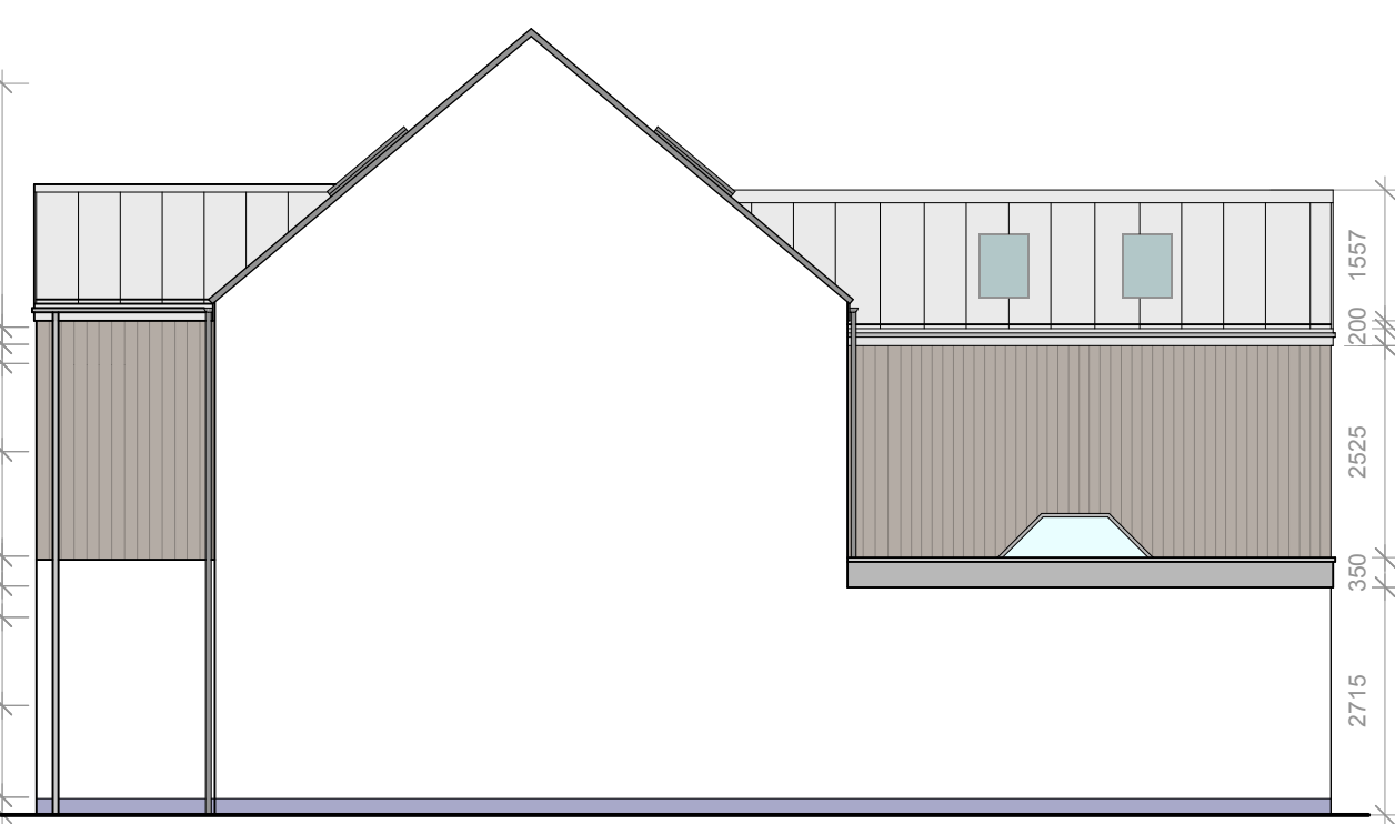
Side Elevation 2
