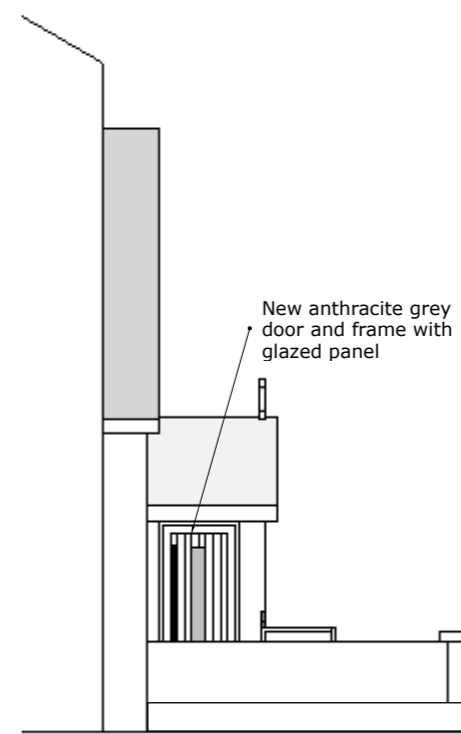
Side Elevation at front
