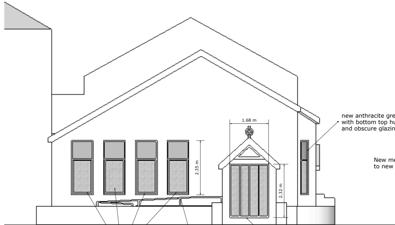
Front Elevation
