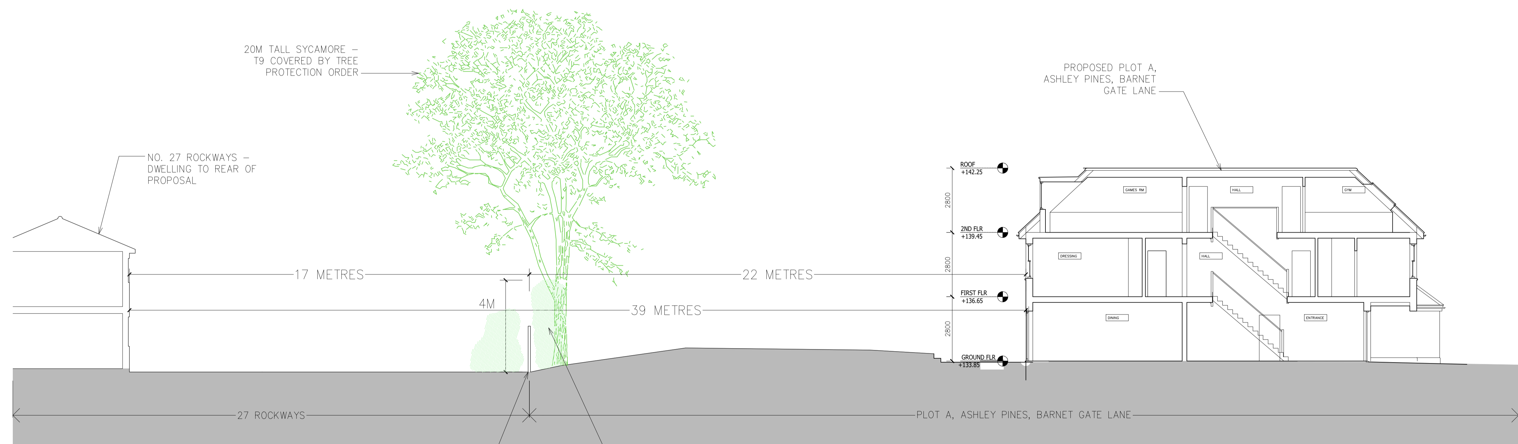
2 PROPOSED LONG SECTION B-B 1 : 100
